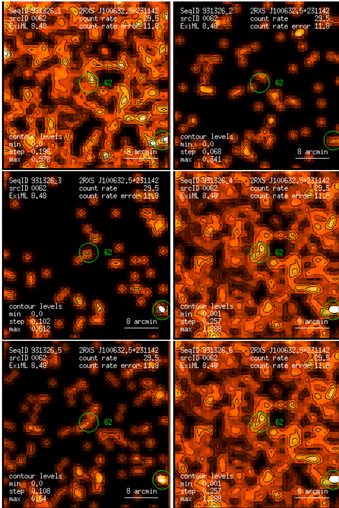
Figure 62: RASS 931326: detection 0062: band rate images, Gaussian filter: (1) PSPC channels 11 – 41, (2) 52 – 90, (3) 91 – 201, (4) 11 – 235, (5) 52 – 201, (6) 11 – 201. Broad band rates in counts/ks. Band rate contour levels in counts/ks/arcmin 2 .
