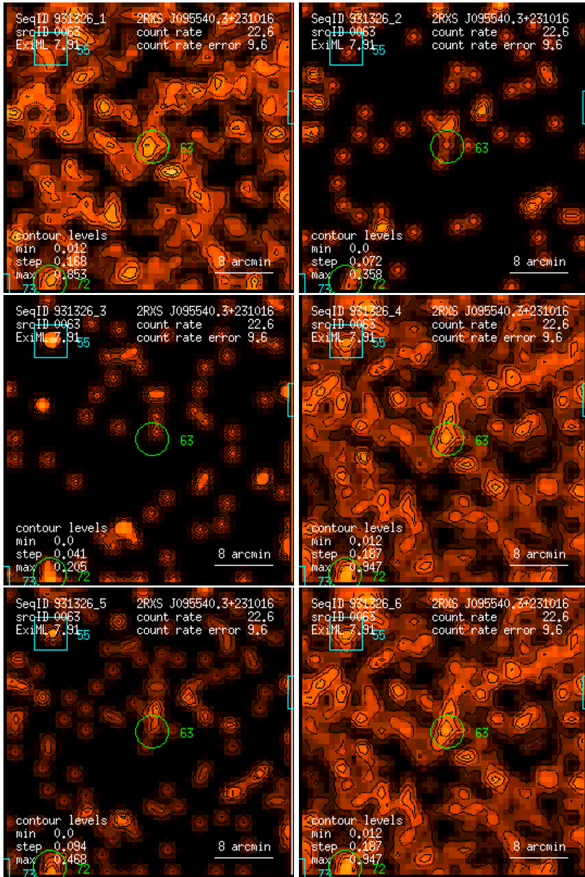
Figure 63: RASS 931326: detection 0063: band rate images, Gaussian filter: (1) PSPC channels 11 – 41, (2) 52 – 90, (3) 91 – 201, (4) 11 – 235, (5) 52 – 201, (6) 11 – 201. Broad band rates in counts/ks. Band rate contour levels in counts/ks/arcmin 2 .
