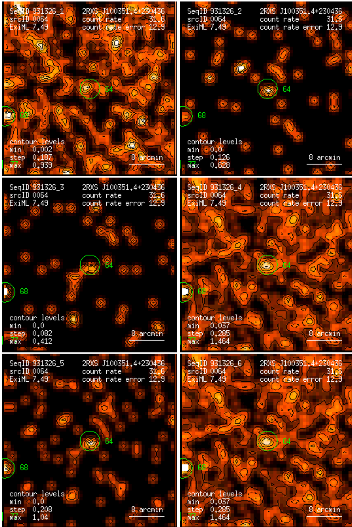
Figure 64: RASS 931326: detection 0064: band rate images, Gaussian filter: (1) PSPC channels 11 – 41, (2) 52 – 90, (3) 91 – 201, (4) 11 – 235, (5) 52 – 201, (6) 11 – 201. Broad band rates in counts/ks. Band rate contour levels in counts/ks/arcmin 2 .
