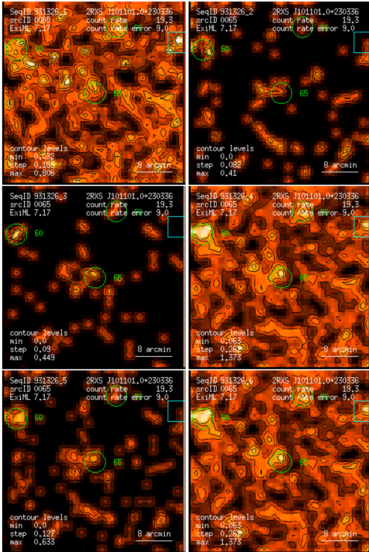
Figure 65: RASS 931326: detection 0065: band rate images, Gaussian filter: (1) PSPC channels 11 – 41, (2) 52 – 90, (3) 91 – 201, (4) 11 – 235, (5) 52 – 201, (6) 11 – 201. Broad band rates in counts/ks. Band rate contour levels in counts/ks/arcmin 2 .
