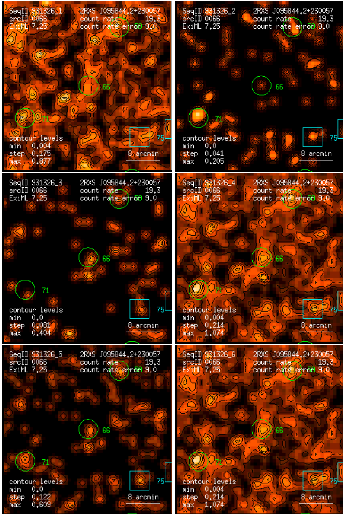
Figure 66: RASS 931326: detection 0066: band rate images, Gaussian filter: (1) PSPC channels 11 – 41, (2) 52 – 90, (3) 91 – 201, (4) 11 – 235, (5) 52 – 201, (6) 11 – 201. Broad band rates in counts/ks. Band rate contour levels in counts/ks/arcmin 2 .
