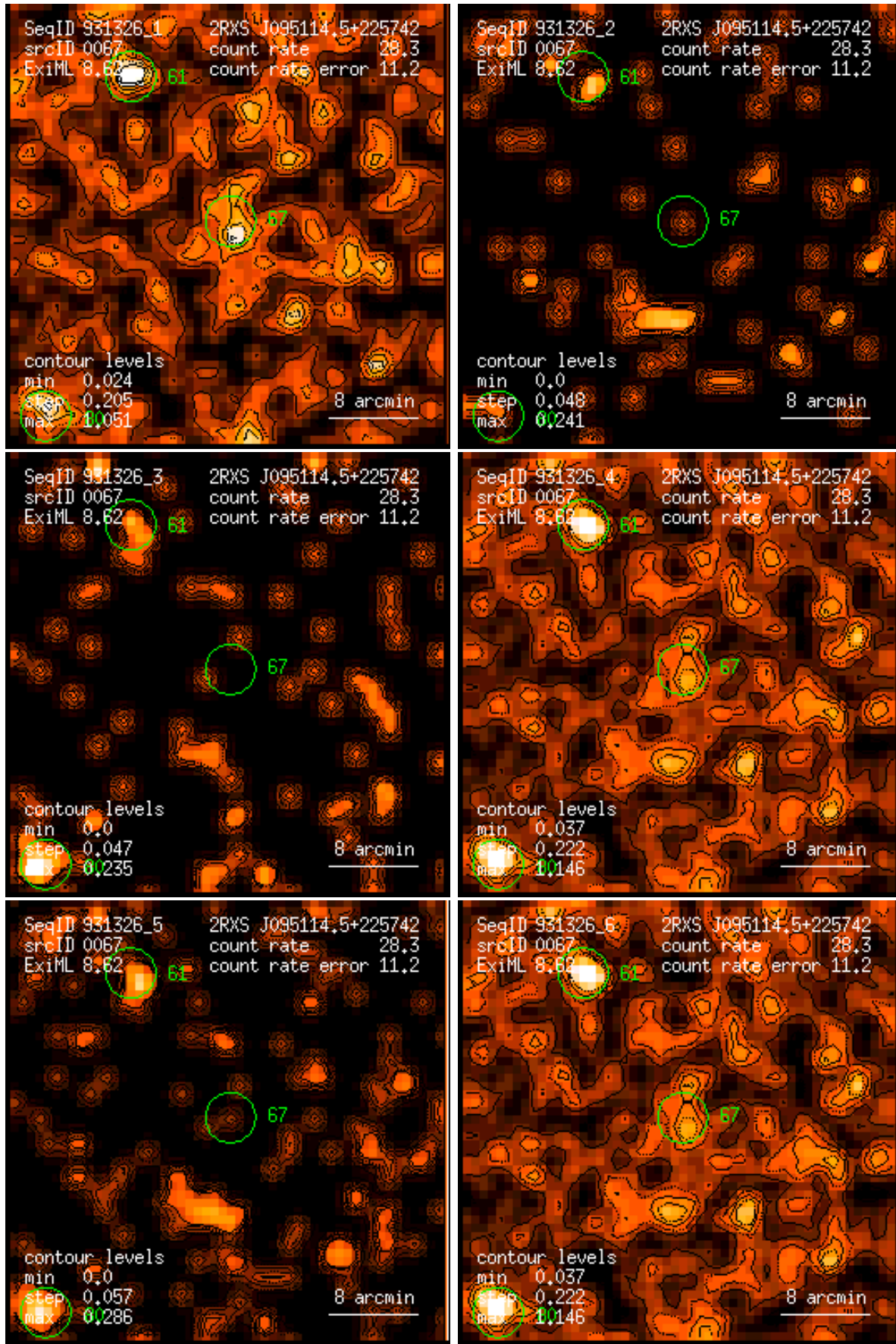
Figure 67: RASS 931326: detection 0067: band rate images, Gaussian filter: (1) PSPC channels 11 – 41, (2) 52 – 90, (3) 91 – 201, (4) 11 – 235, (5) 52 – 201, (6) 11 – 201. Broad band rates in counts/ks. Band rate contour levels in counts/ks/arcmin 2 .
