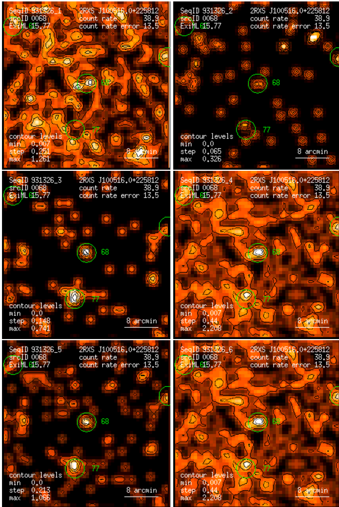
Figure 68: RASS 931326: detection 0068: band rate images, Gaussian filter: (1) PSPC channels 11 – 41, (2) 52 – 90, (3) 91 – 201, (4) 11 – 235, (5) 52 – 201, (6) 11 – 201. Broad band rates in counts/ks. Band rate contour levels in counts/ks/arcmin 2 .
