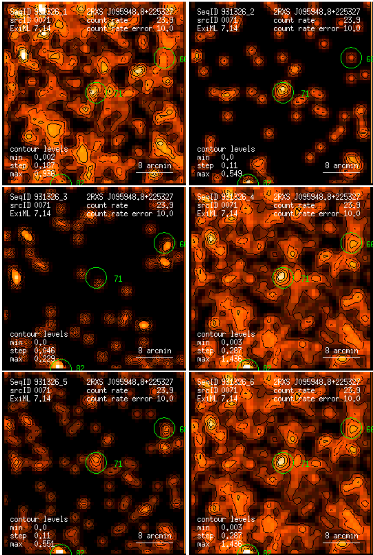
Figure 71: RASS 931326: detection 0071: band rate images, Gaussian filter: (1) PSPC channels 11 – 41, (2) 52 – 90, (3) 91 – 201, (4) 11 – 235, (5) 52 – 201, (6) 11 – 201. Broad band rates in counts/ks. Band rate contour levels in counts/ks/arcmin 2 .
