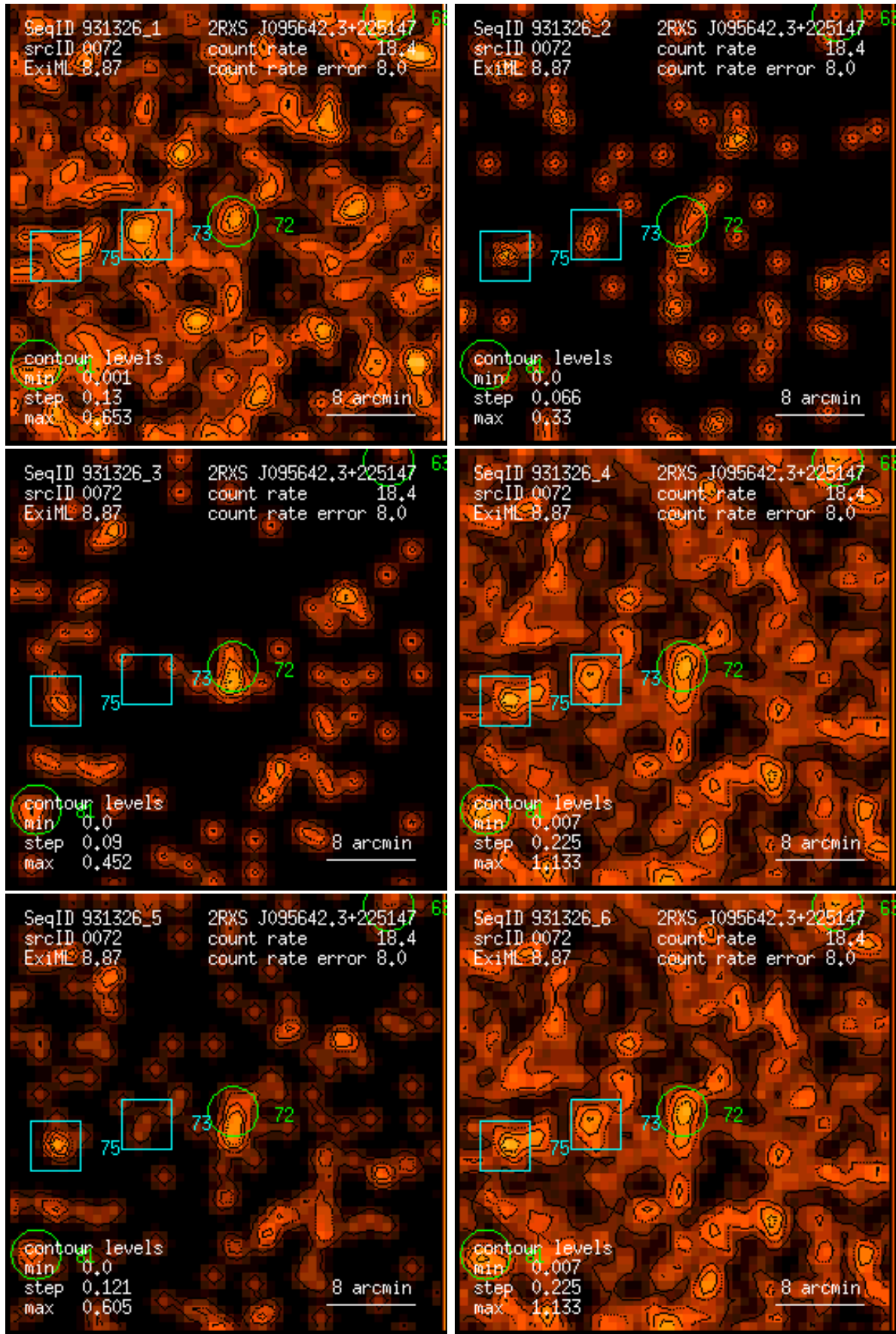
Figure 72: RASS 931326: detection 0072: band rate images, Gaussian filter: (1) PSPC channels 11 – 41, (2) 52 – 90, (3) 91 – 201, (4) 11 – 235, (5) 52 – 201, (6) 11 – 201. Broad band rates in counts/ks. Band rate contour levels in counts/ks/arcmin 2 .
