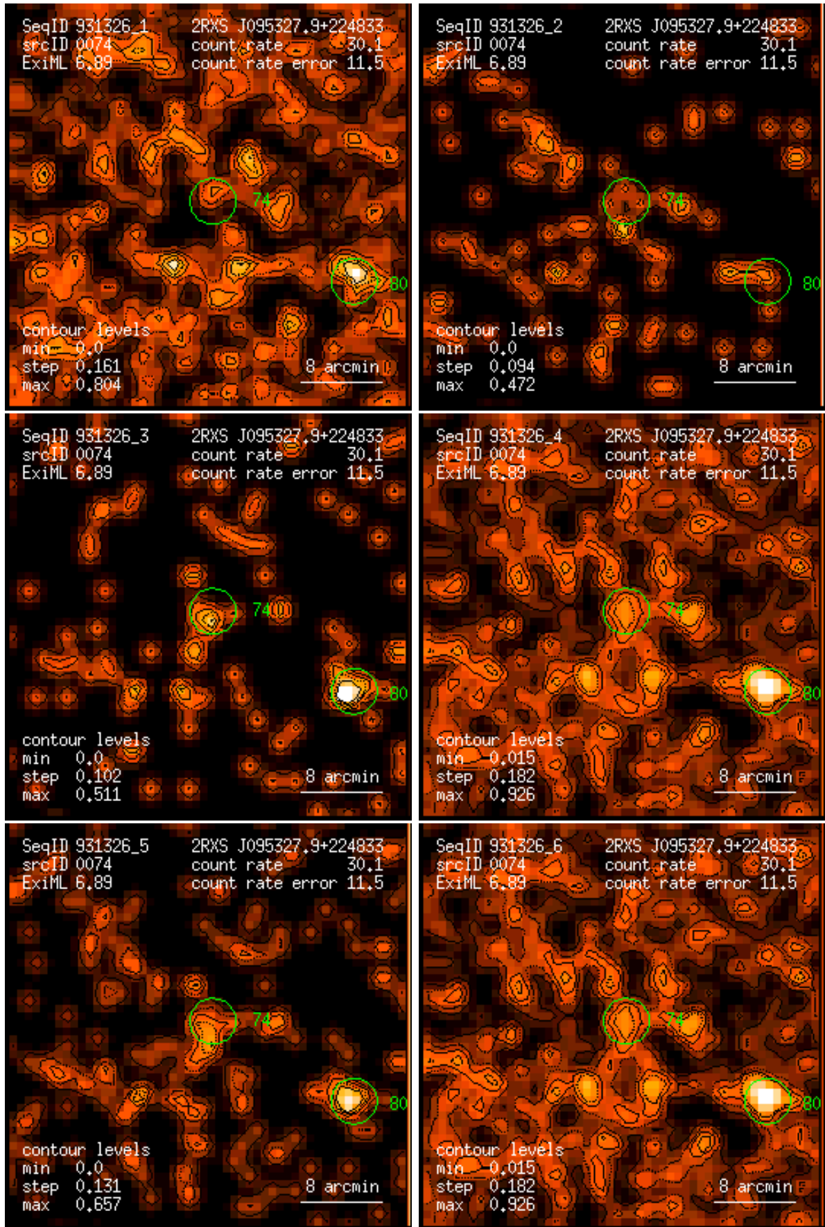
Figure 74: RASS 931326: detection 0074: band rate images, Gaussian filter: (1) PSPC channels 11 – 41, (2) 52 – 90, (3) 91 – 201, (4) 11 – 235, (5) 52 – 201, (6) 11 – 201. Broad band rates in counts/ks. Band rate contour levels in counts/ks/arcmin 2 .
