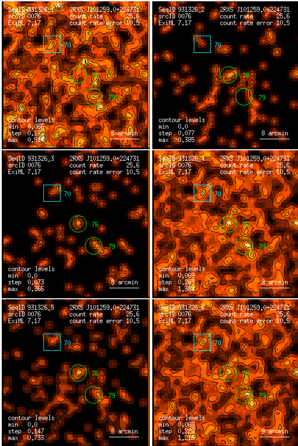
Figure 76: RASS 931326: detection 0076: band rate images, Gaussian filter: (1) PSPC channels 11 – 41, (2) 52 – 90, (3) 91 – 201, (4) 11 – 235, (5) 52 – 201, (6) 11 – 201. Broad band rates in counts/ks. Band rate contour levels in counts/ks/arcmin 2 .
