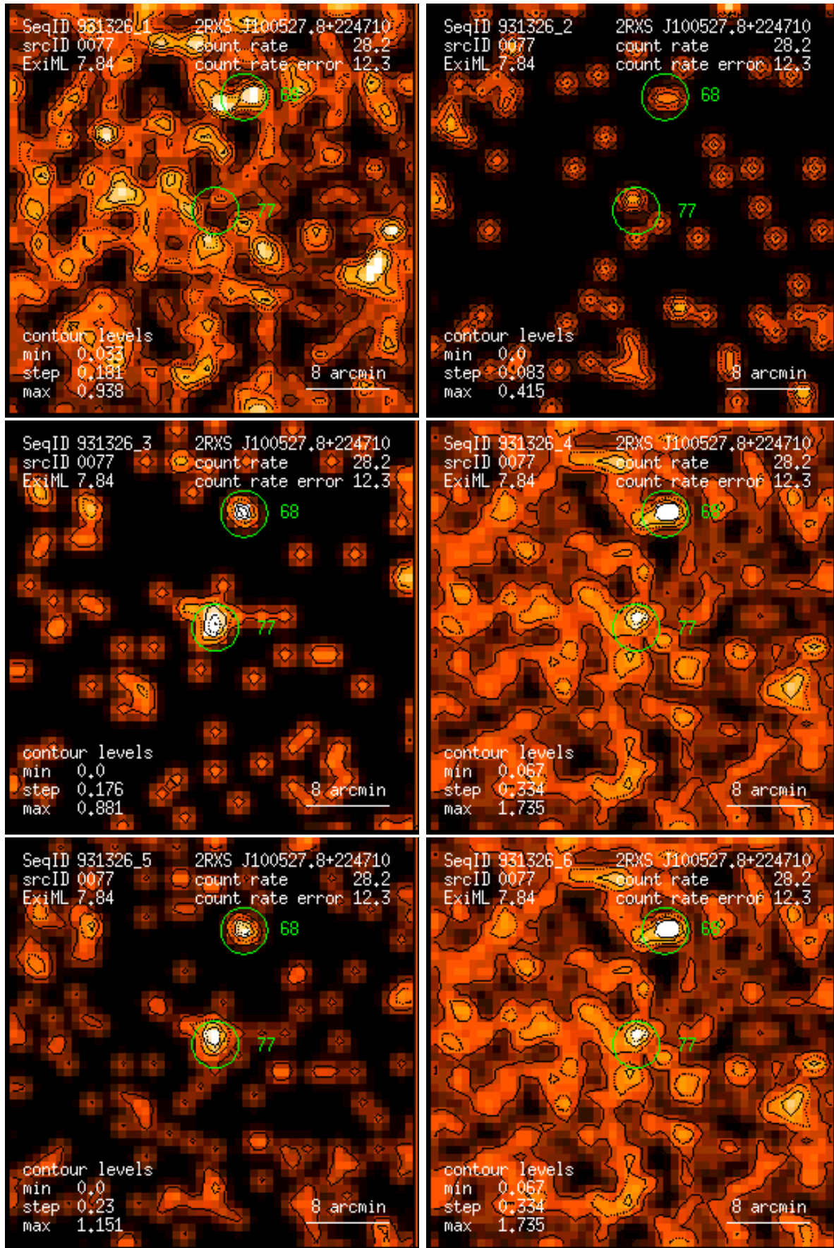
Figure 77: RASS 931326: detection 0077: band rate images, Gaussian filter: (1) PSPC channels 11 – 41, (2) 52 – 90, (3) 91 – 201, (4) 11 – 235, (5) 52 – 201, (6) 11 – 201. Broad band rates in counts/ks. Band rate contour levels in counts/ks/arcmin 2 .
