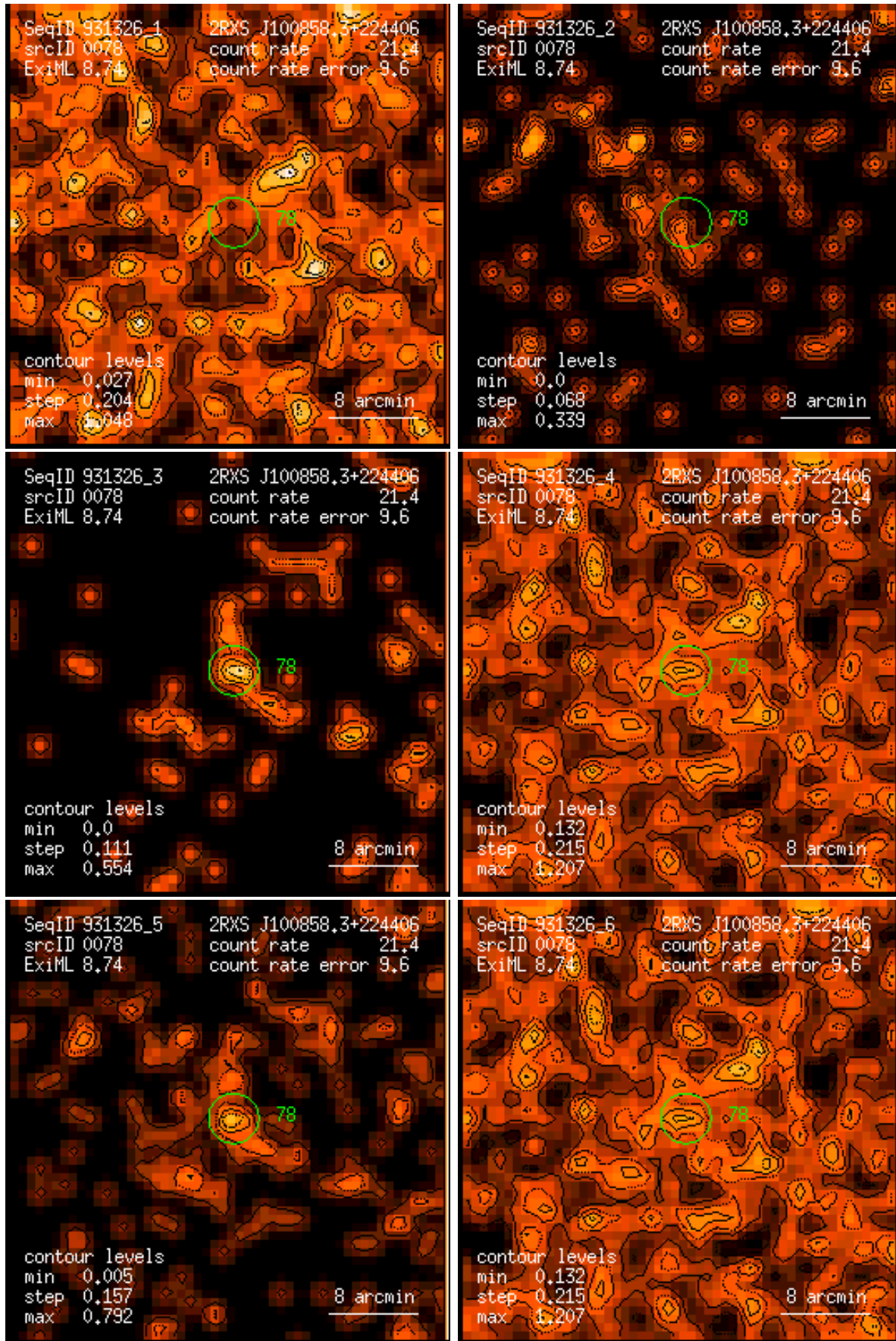
Figure 78: RASS 931326: detection 0078: band rate images, Gaussian filter: (1) PSPC channels 11 – 41, (2) 52 – 90, (3) 91 – 201, (4) 11 – 235, (5) 52 – 201, (6) 11 – 201. Broad band rates in counts/ks. Band rate contour levels in counts/ks/arcmin 2 .
