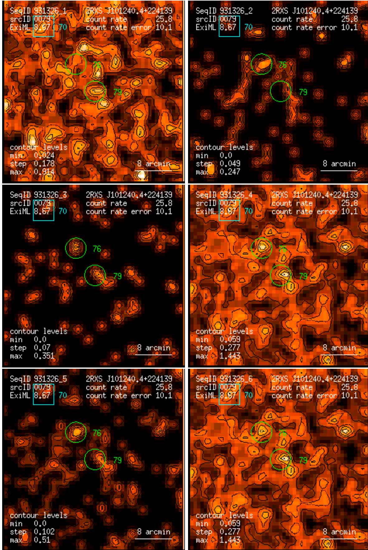
Figure 79: RASS 931326: detection 0079: band rate images, Gaussian filter: (1) PSPC channels 11 – 41, (2) 52 – 90, (3) 91 – 201, (4) 11 – 235, (5) 52 – 201, (6) 11 – 201. Broad band rates in counts/ks. Band rate contour levels in counts/ks/arcmin 2 .
