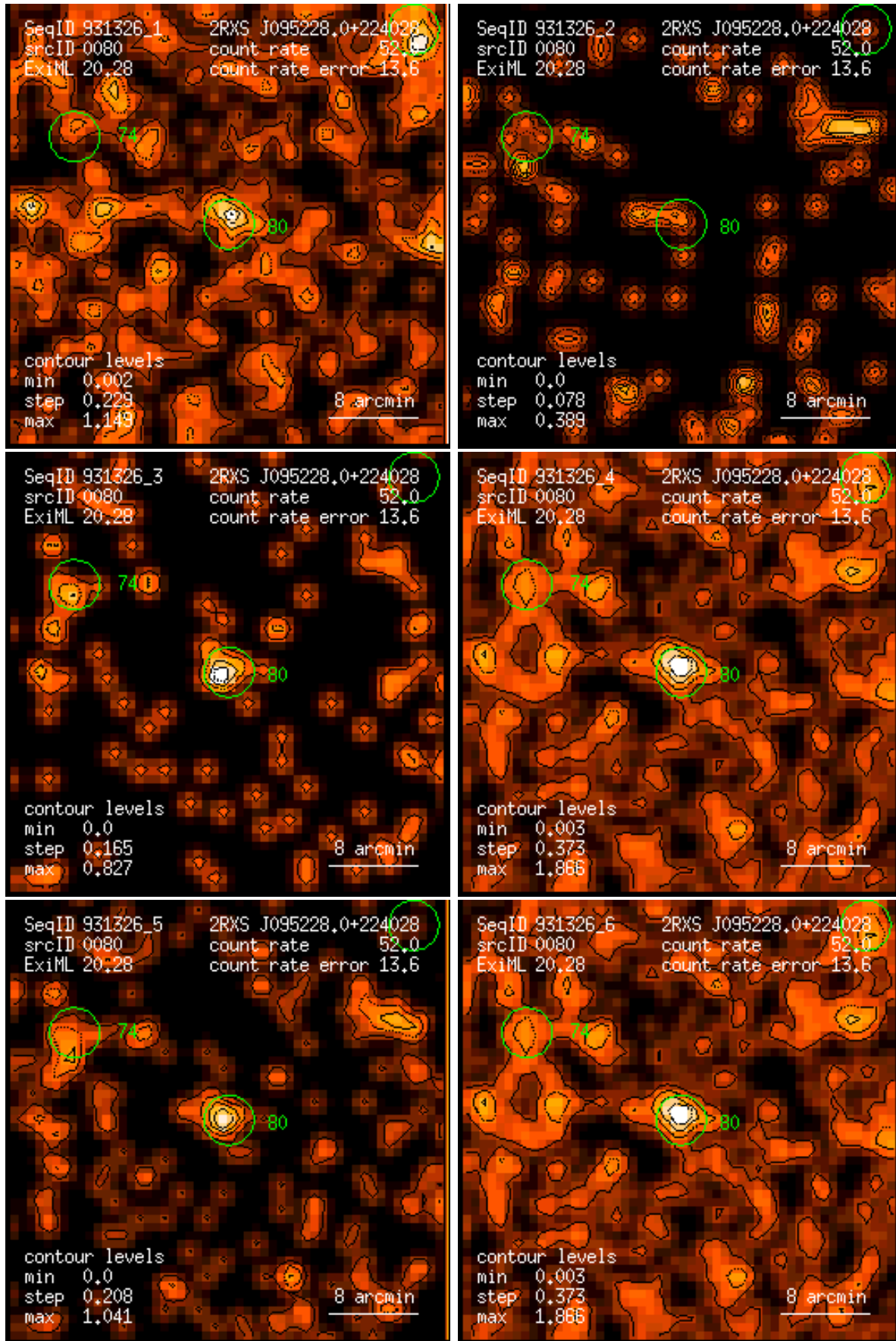
Figure 80: RASS 931326: detection 0080: band rate images, Gaussian filter: (1) PSPC channels 11 – 41, (2) 52 – 90, (3) 91 – 201, (4) 11 – 235, (5) 52 – 201, (6) 11 – 201. Broad band rates in counts/ks. Band rate contour levels in counts/ks/arcmin 2 .
