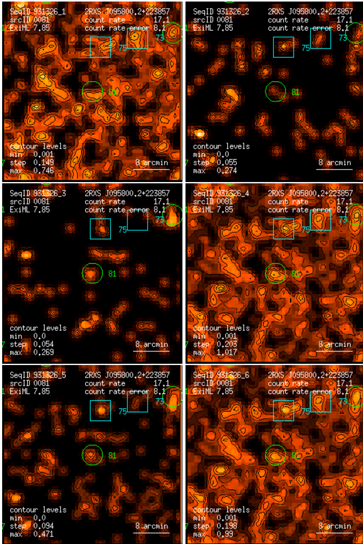
Figure 81: RASS 931326: detection 0081: band rate images, Gaussian filter: (1) PSPC channels 11 – 41, (2) 52 – 90, (3) 91 – 201, (4) 11 – 235, (5) 52 – 201, (6) 11 – 201. Broad band rates in counts/ks. Band rate contour levels in counts/ks/arcmin 2 .
