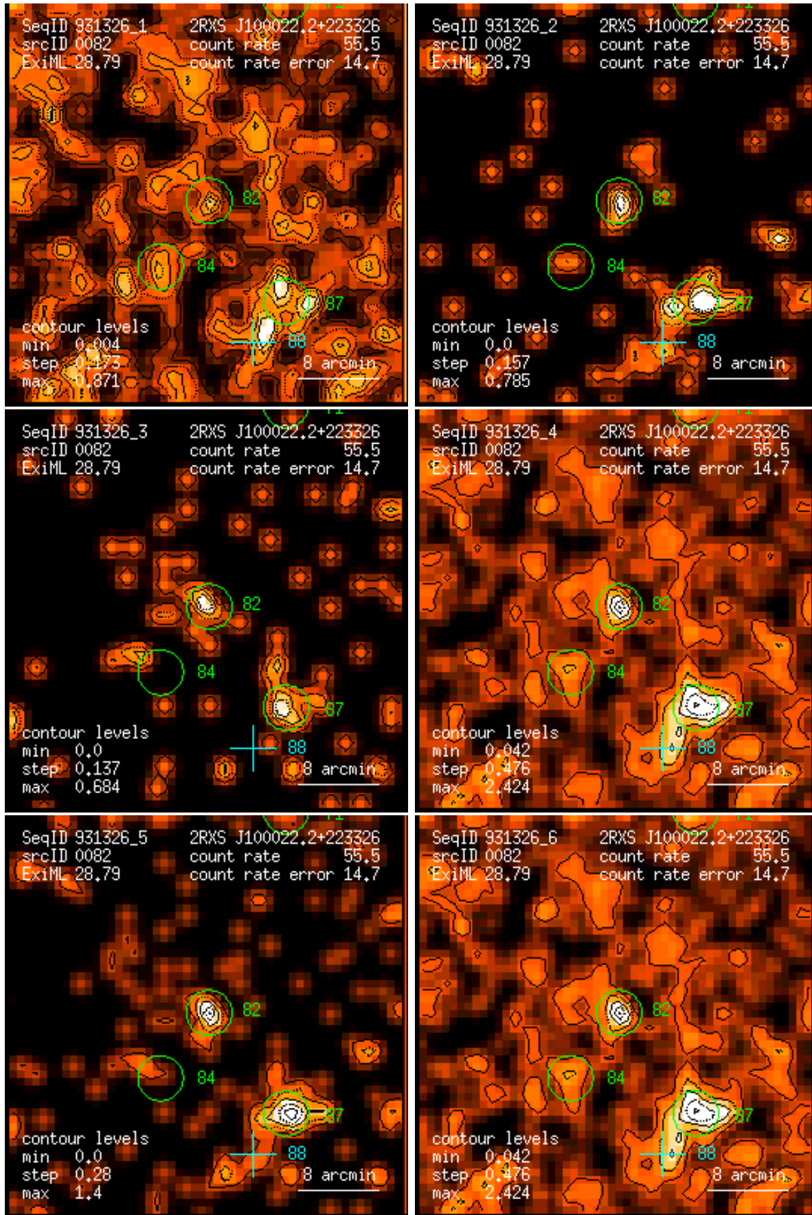
Figure 82: RASS 931326: detection 0082: band rate images, Gaussian filter: (1) PSPC channels 11 – 41, (2) 52 – 90, (3) 91 – 201, (4) 11 – 235, (5) 52 – 201, (6) 11 – 201. Broad band rates in counts/ks. Band rate contour levels in counts/ks/arcmin 2 .
