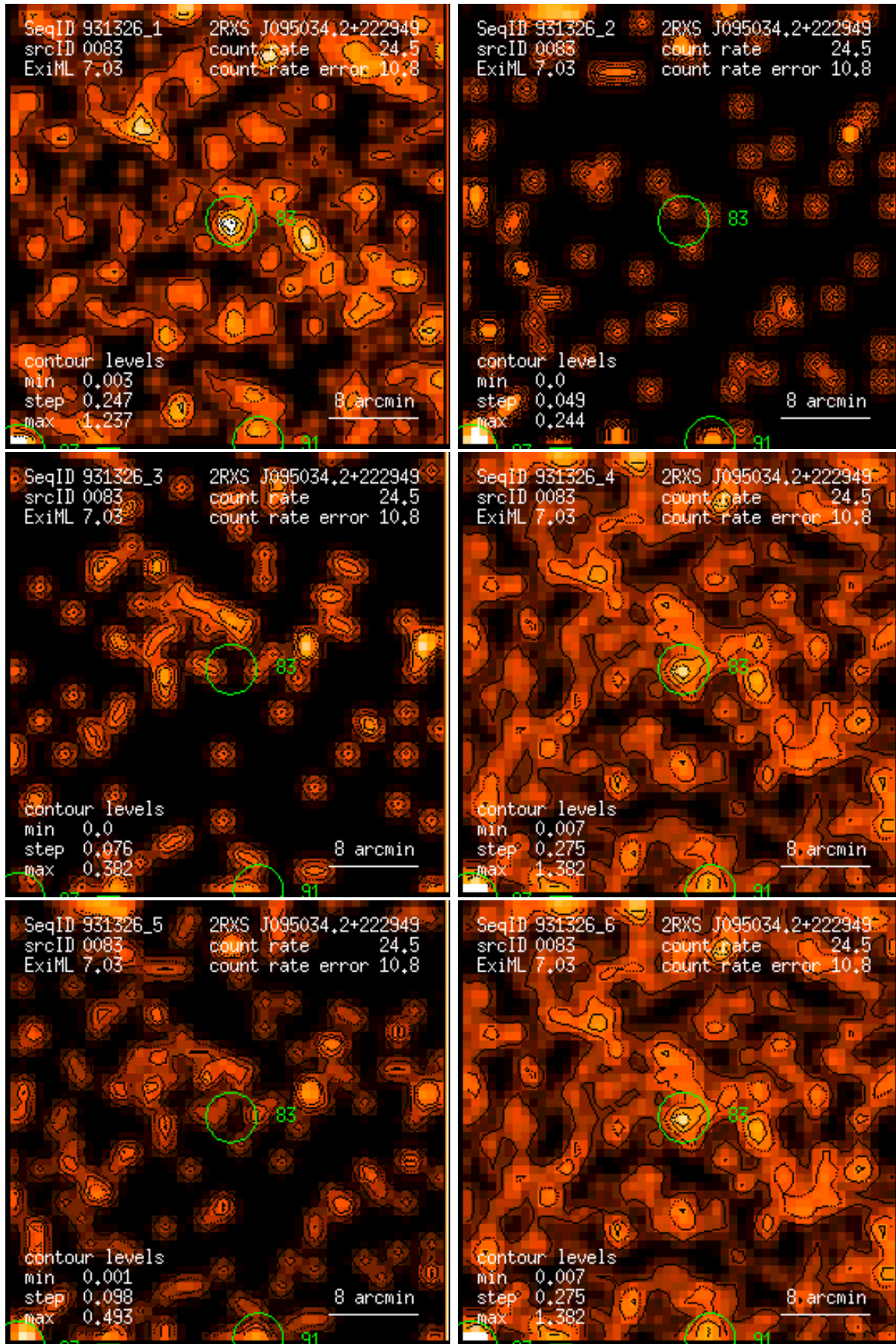
Figure 83: RASS 931326: detection 0083: band rate images, Gaussian filter: (1) PSPC channels 11 – 41, (2) 52 – 90, (3) 91 – 201, (4) 11 – 235, (5) 52 – 201, (6) 11 – 201. Broad band rates in counts/ks. Band rate contour levels in counts/ks/arcmin 2 .
