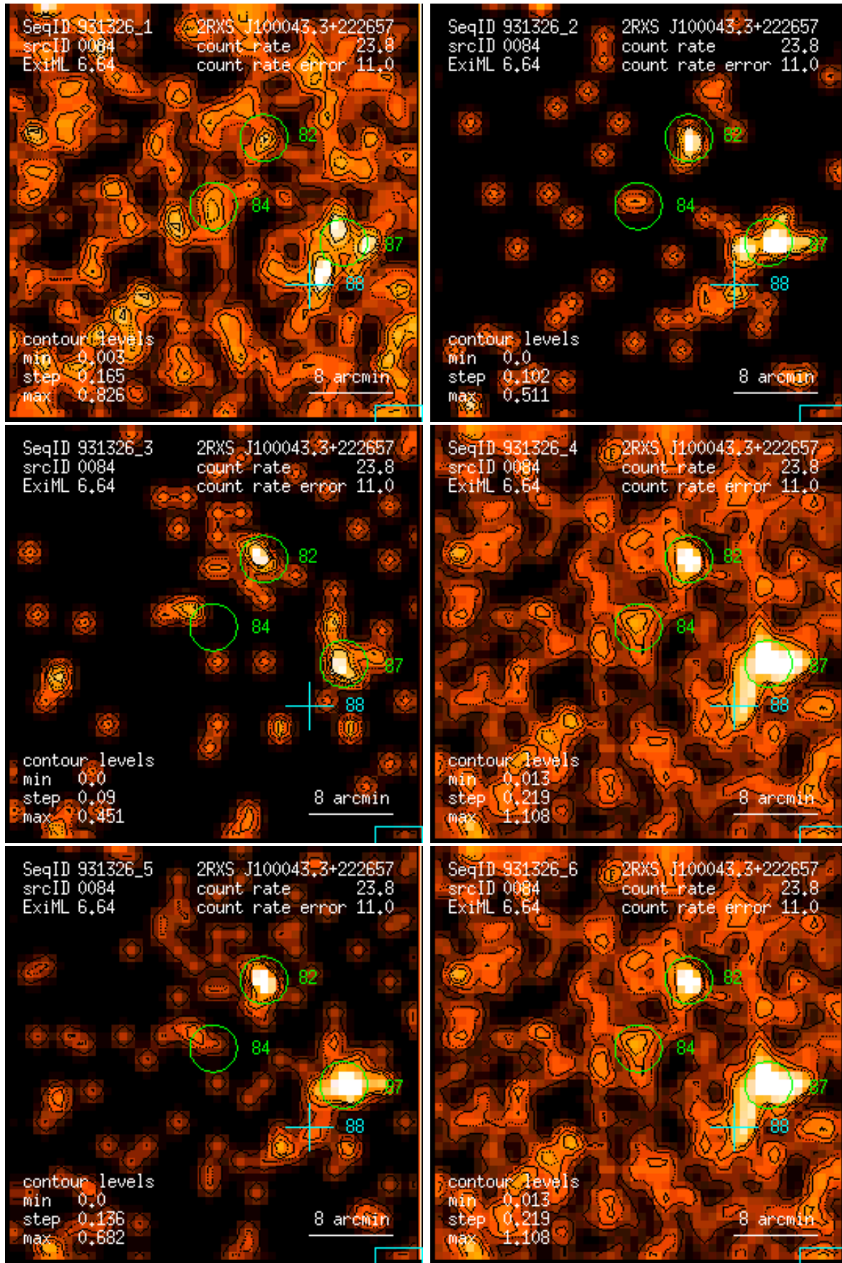
Figure 84: RASS 931326: detection 0084: band rate images, Gaussian filter: (1) PSPC channels 11 – 41, (2) 52 – 90, (3) 91 – 201, (4) 11 – 235, (5) 52 – 201, (6) 11 – 201. Broad band rates in counts/ks. Band rate contour levels in counts/ks/arcmin 2 .
