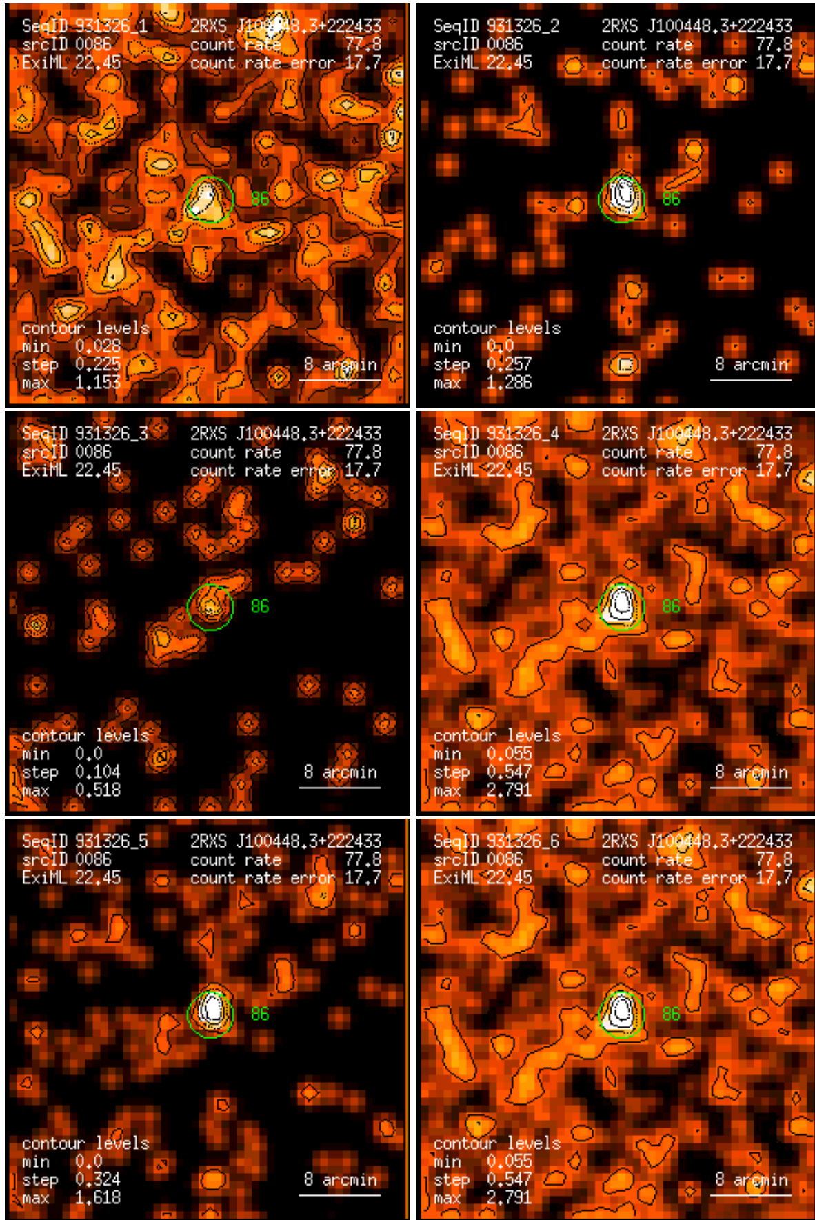
Figure 86: RASS 931326: detection 0086: band rate images, Gaussian filter: (1) PSPC channels 11 – 41, (2) 52 – 90, (3) 91 – 201, (4) 11 – 235, (5) 52 – 201, (6) 11 – 201. Broad band rates in counts/ks. Band rate contour levels in counts/ks/arcmin 2 .
