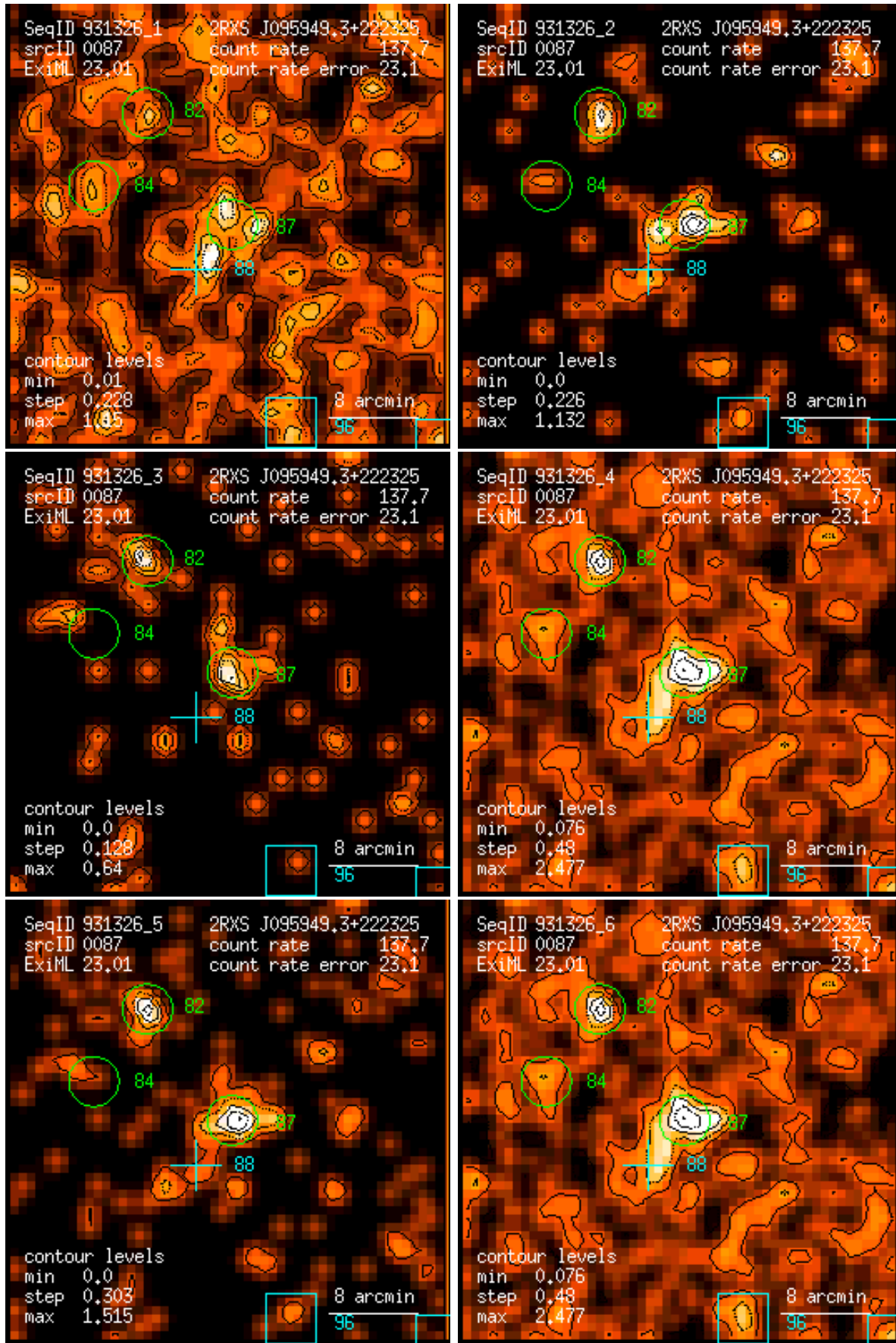
Figure 87: RASS 931326: detection 0087: band rate images, Gaussian filter: (1) PSPC channels 11 – 41, (2) 52 – 90, (3) 91 – 201, (4) 11 – 235, (5) 52 – 201, (6) 11 – 201. Broad band rates in counts/ks. Band rate contour levels in counts/ks/arcmin 2 .
