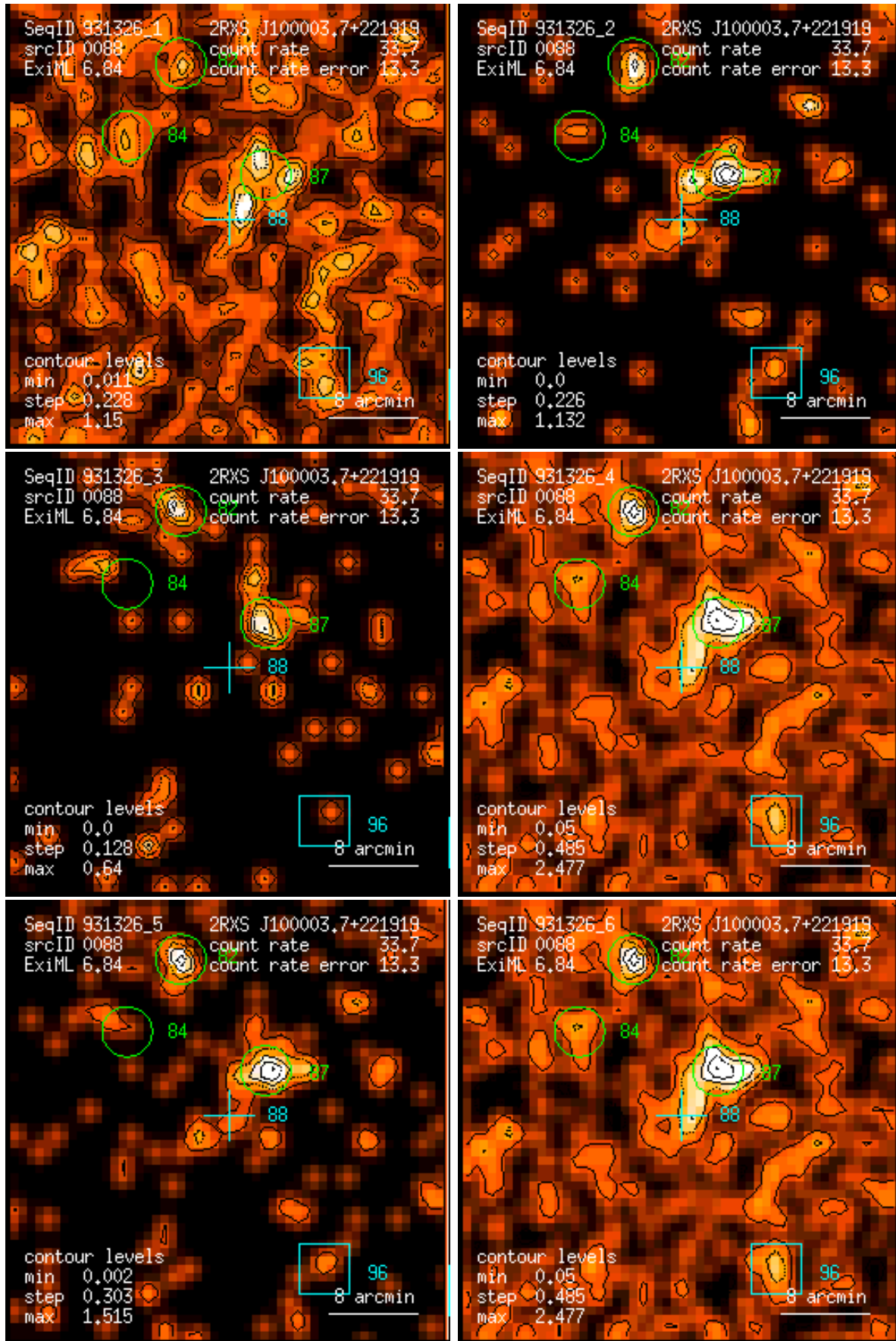
Figure 88: RASS 931326: detection 0088: band rate images, Gaussian filter: (1) PSPC channels 11 – 41, (2) 52 – 90, (3) 91 – 201, (4) 11 – 235, (5) 52 – 201, (6) 11 – 201. Broad band rates in counts/ks. Band rate contour levels in counts/ks/arcmin 2 .
