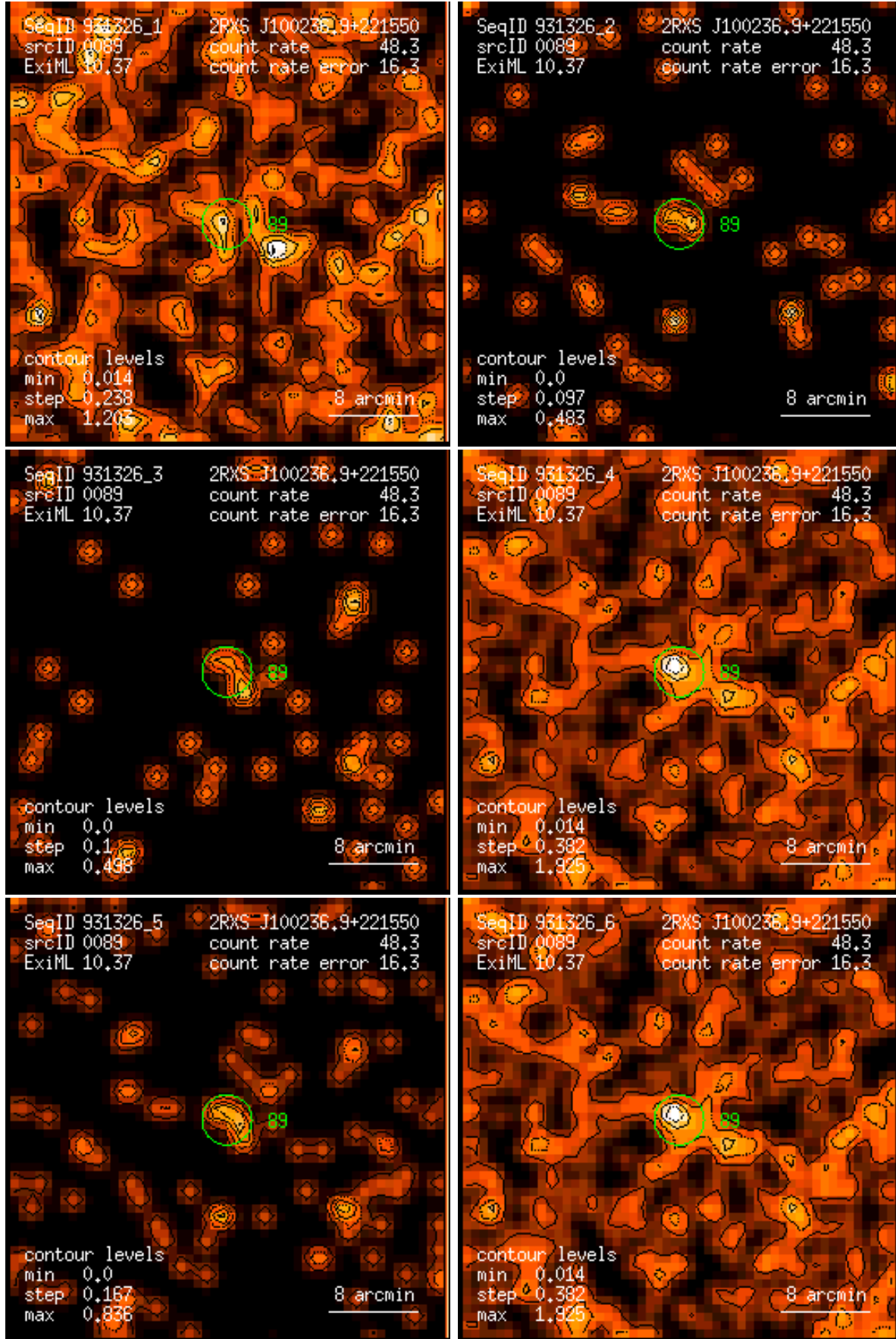
Figure 89: RASS 931326: detection 0089: band rate images, Gaussian filter: (1) PSPC channels 11 – 41, (2) 52 – 90, (3) 91 – 201, (4) 11 – 235, (5) 52 – 201, (6) 11 – 201. Broad band rates in counts/ks. Band rate contour levels in counts/ks/arcmin 2 .
