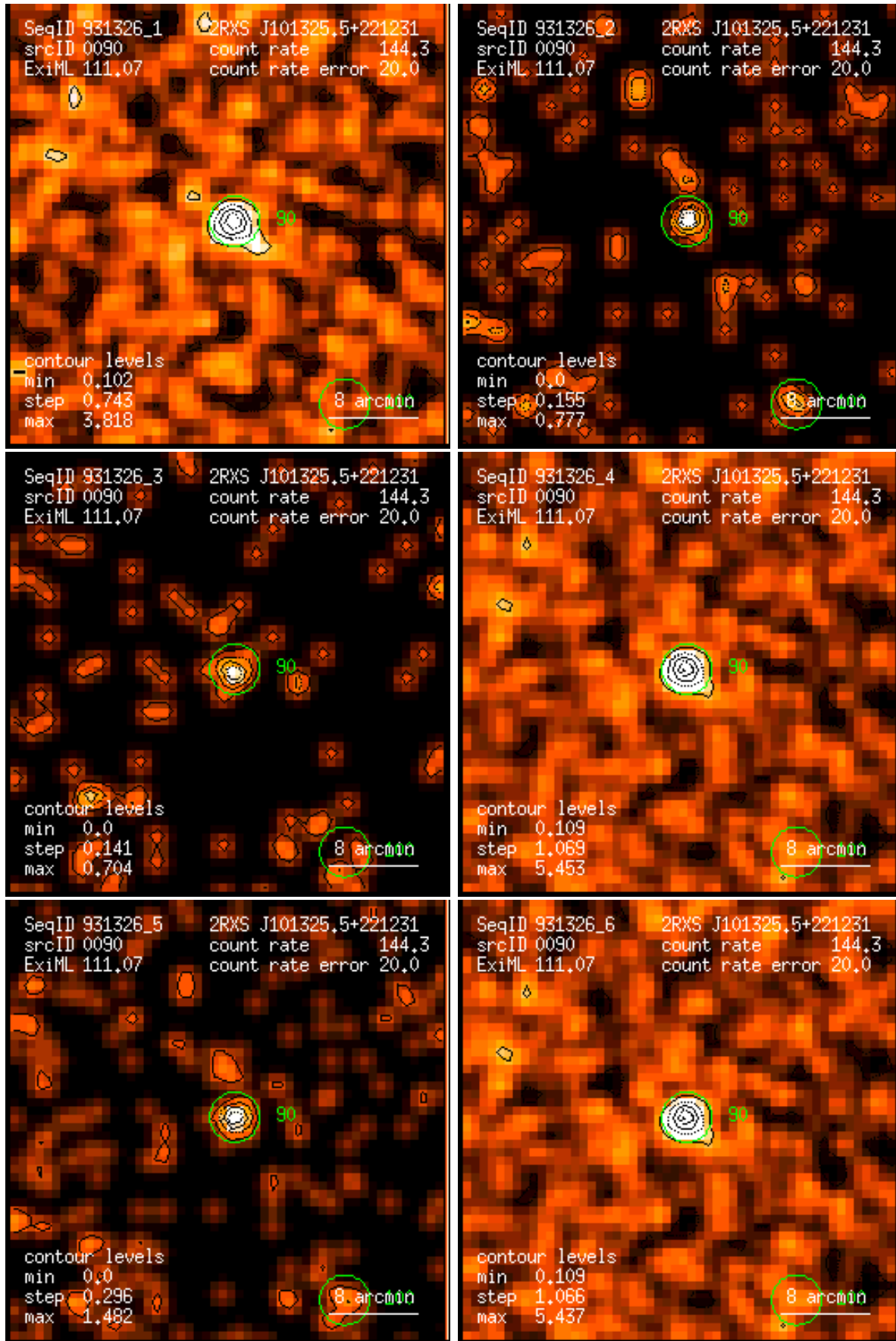
Figure 90: RASS 931326: detection 0090: band rate images, Gaussian filter: (1) PSPC channels 11 – 41, (2) 52 – 90, (3) 91 – 201, (4) 11 – 235, (5) 52 – 201, (6) 11 – 201. Broad band rates in counts/ks. Band rate contour levels in counts/ks/arcmin 2 .
