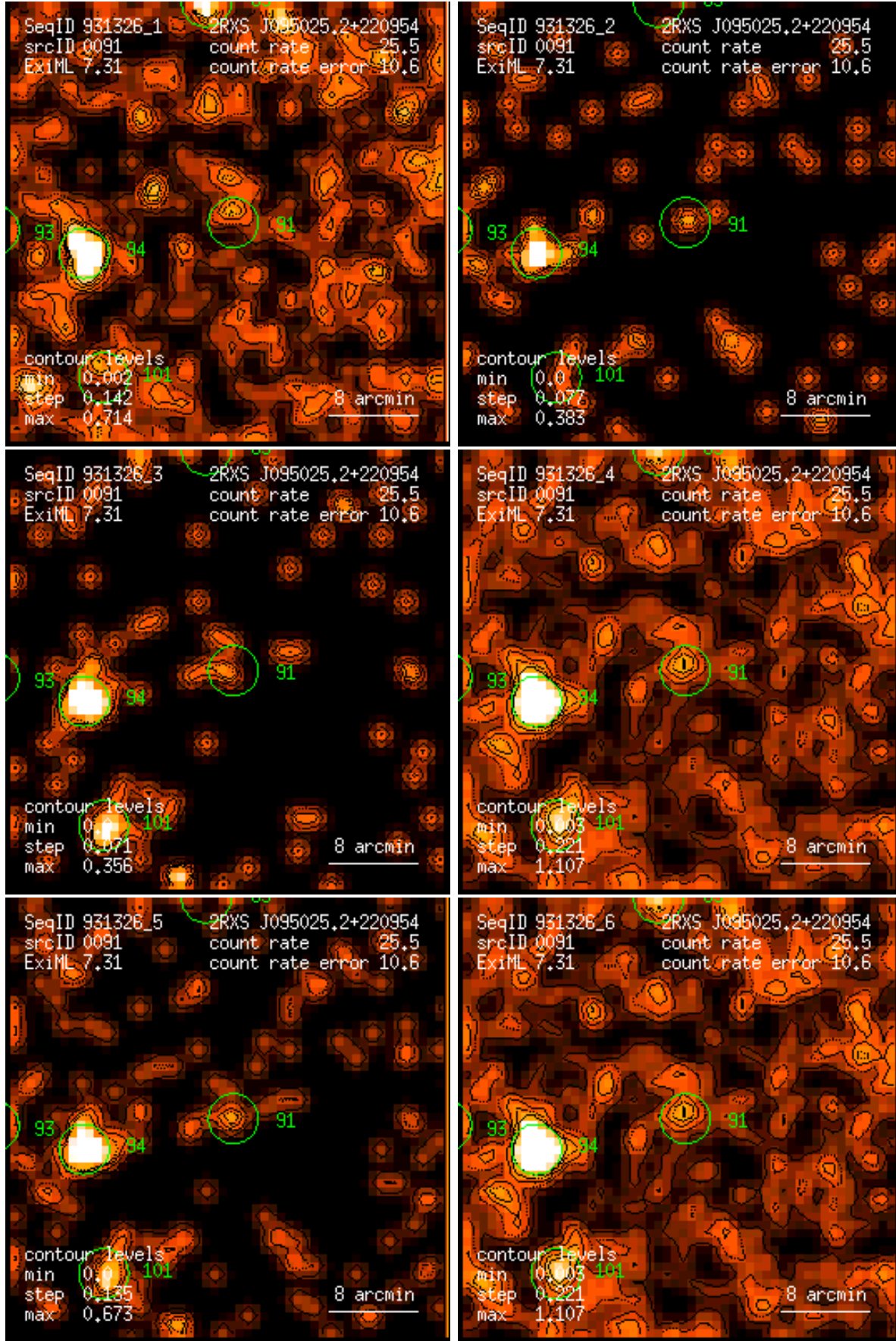
Figure 91: RASS 931326: detection 0091: band rate images, Gaussian filter: (1) PSPC channels 11 – 41, (2) 52 – 90, (3) 91 – 201, (4) 11 – 235, (5) 52 – 201, (6) 11 – 201. Broad band rates in counts/ks. Band rate contour levels in counts/ks/arcmin 2 .
