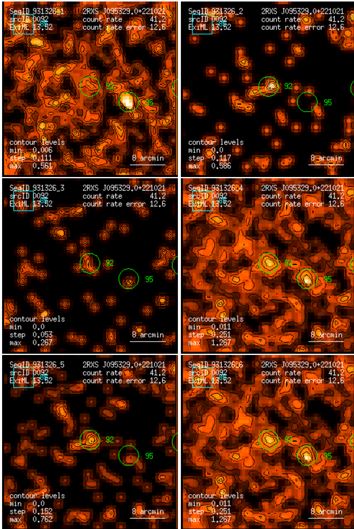
Figure 92: RASS 931326: detection 0092: band rate images, Gaussian filter: (1) PSPC channels 11 – 41, (2) 52 – 90, (3) 91 – 201, (4) 11 – 235, (5) 52 – 201, (6) 11 – 201. Broad band rates in counts/ks. Band rate contour levels in counts/ks/arcmin 2 .
