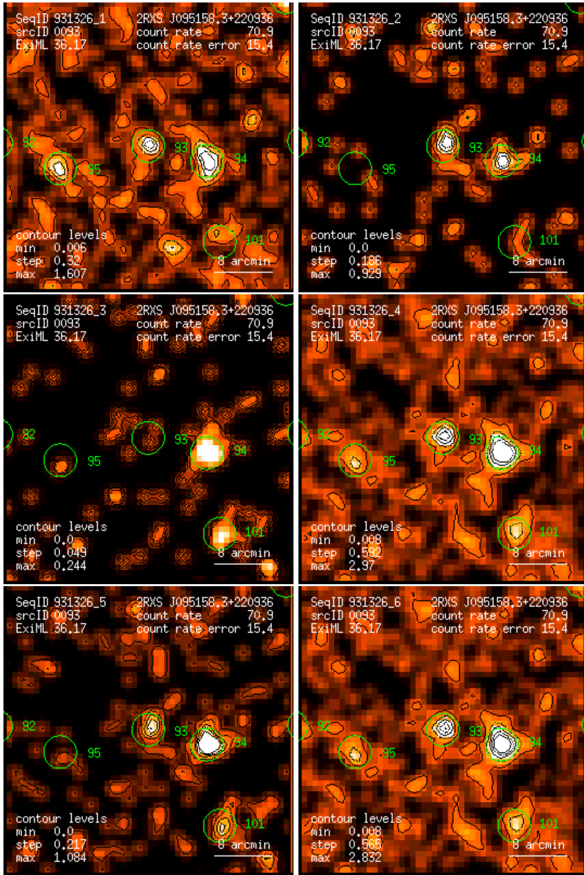
Figure 93: RASS 931326: detection 0093: band rate images, Gaussian filter: (1) PSPC channels 11 – 41, (2) 52 – 90, (3) 91 – 201, (4) 11 – 235, (5) 52 – 201, (6) 11 – 201. Broad band rates in counts/ks. Band rate contour levels in counts/ks/arcmin 2 .
