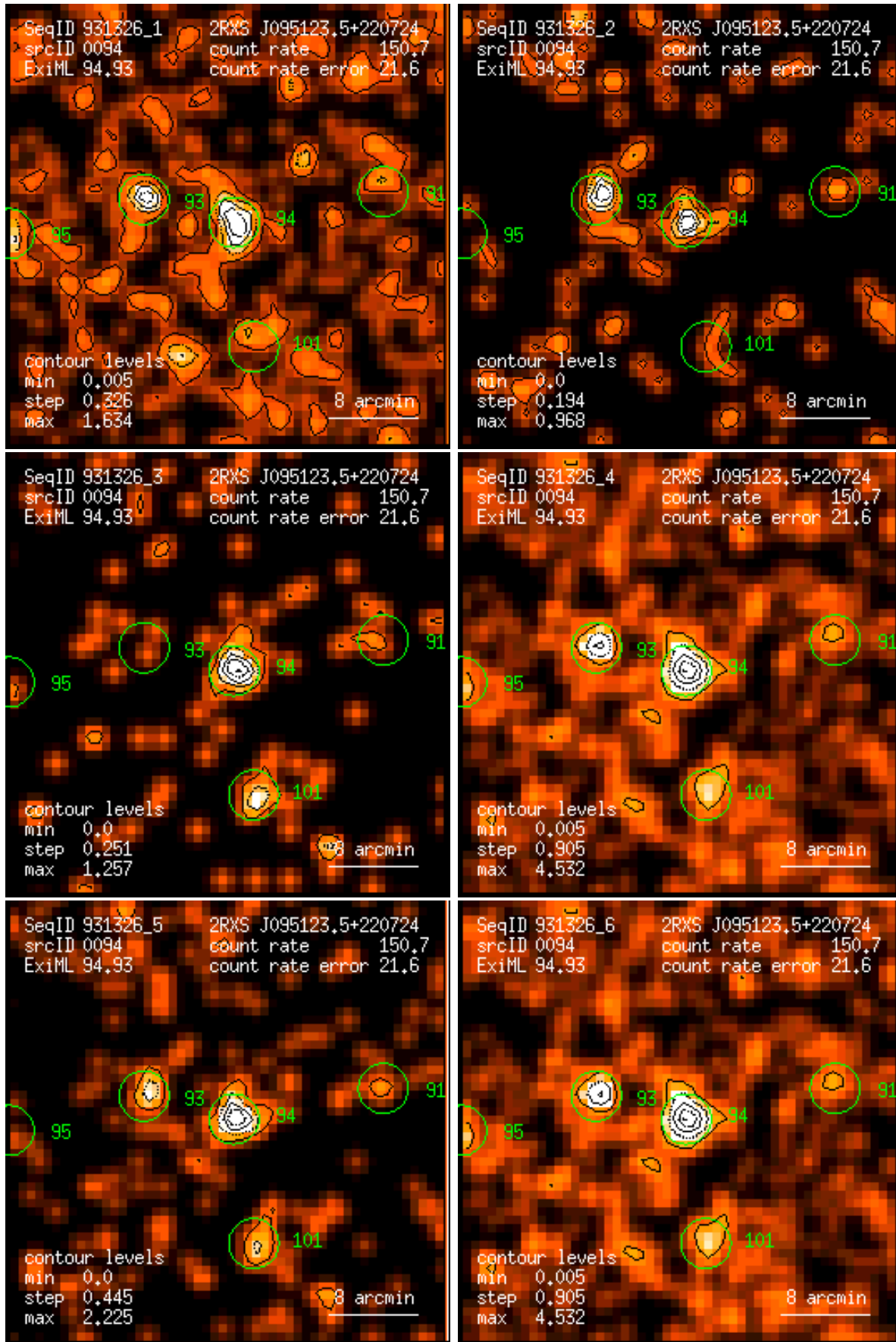
Figure 94: RASS 931326: detection 0094: band rate images, Gaussian filter: (1) PSPC channels 11 – 41, (2) 52 – 90, (3) 91 – 201, (4) 11 – 235, (5) 52 – 201, (6) 11 – 201. Broad band rates in counts/ks. Band rate contour levels in counts/ks/arcmin 2 .
