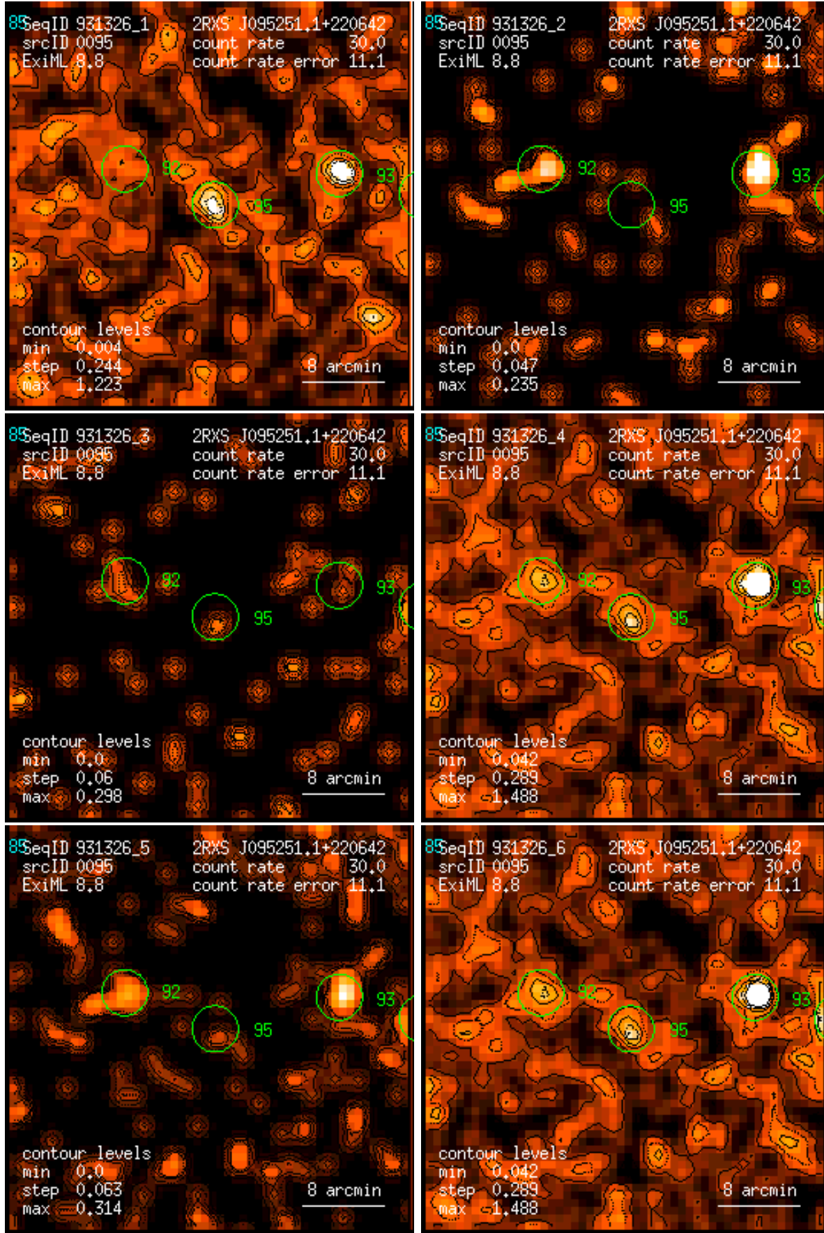
Figure 95: RASS 931326: detection 0095: band rate images, Gaussian filter: (1) PSPC channels 11 – 41, (2) 52 – 90, (3) 91 – 201, (4) 11 – 235, (5) 52 – 201, (6) 11 – 201. Broad band rates in counts/ks. Band rate contour levels in counts/ks/arcmin 2 .
