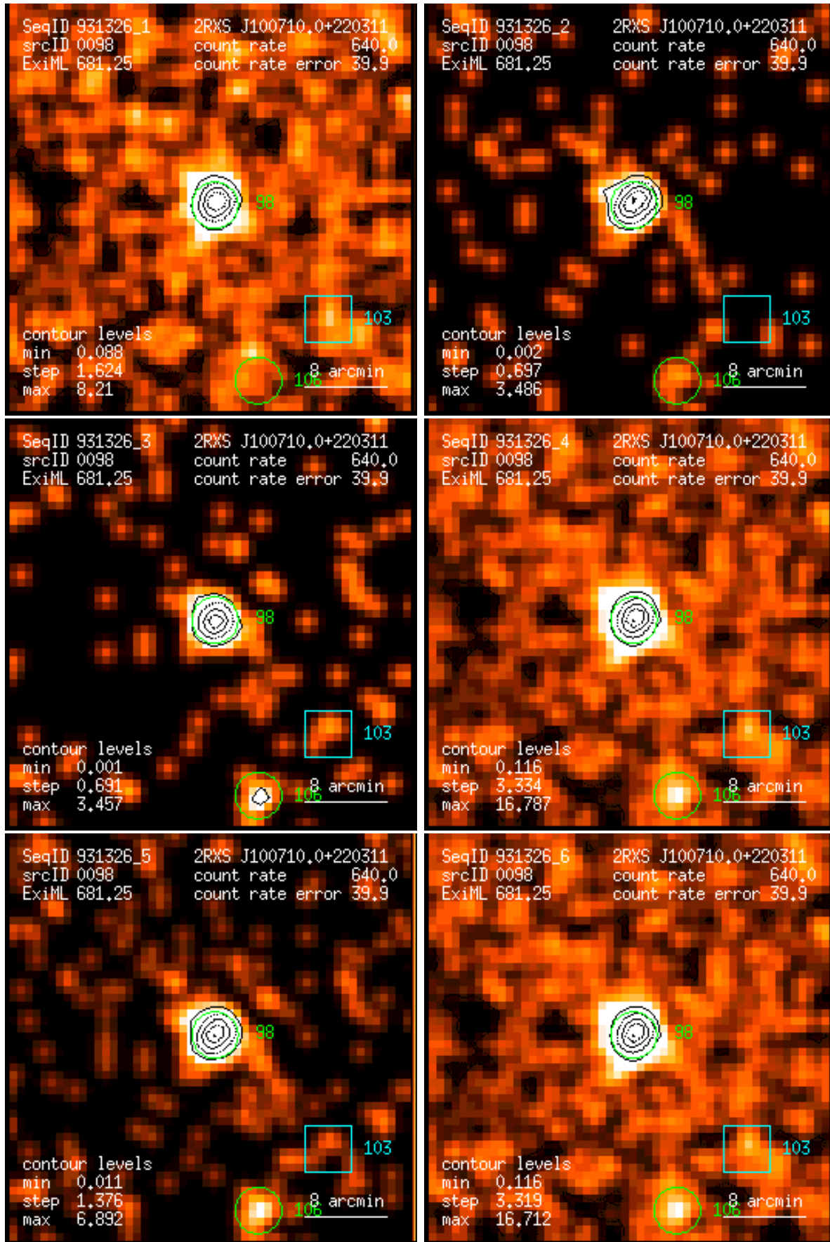
Figure 98: RASS 931326: detection 0098: band rate images, Gaussian filter: (1) PSPC channels 11 – 41, (2) 52 – 90, (3) 91 – 201, (4) 11 – 235, (5) 52 – 201, (6) 11 – 201. Broad band rates in counts/ks. Band rate contour levels in counts/ks/arcmin 2 .
