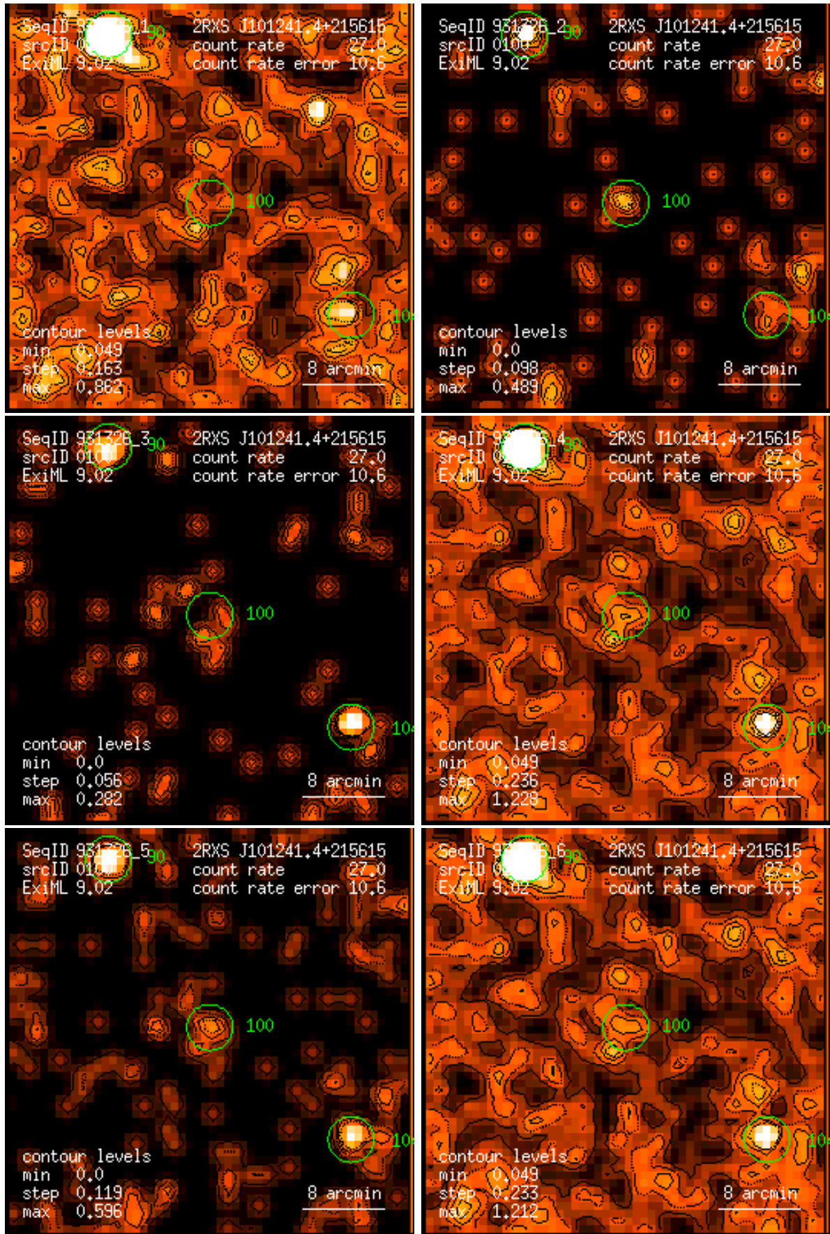
Figure 100: RASS 931326: detection 0100: band rate images, Gaussian filter: (1) PSPC channels 11 – 41, (2) 52 – 90, (3) 91 – 201, (4) 11 – 235, (5) 52 – 201, (6) 11 – 201. Broad band rates in counts/ks. Band rate contour levels in counts/ks/arcmin 2 .
