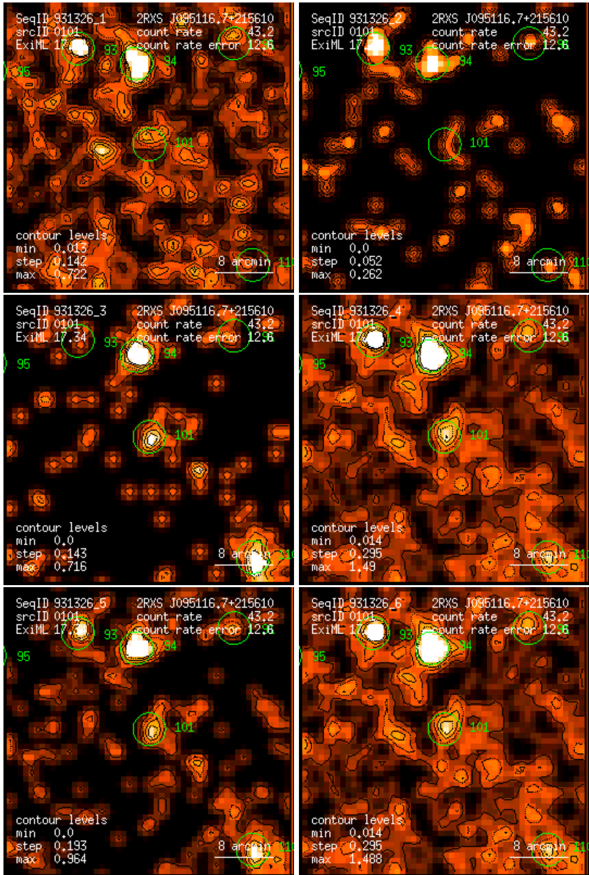
Figure 101: RASS 931326: detection 0101: band rate images, Gaussian filter: (1) PSPC channels 11 – 41, (2) 52 – 90, (3) 91 – 201, (4) 11 – 235, (5) 52 – 201, (6) 11 – 201. Broad band rates in counts/ks. Band rate contour levels in counts/ks/arcmin 2 .
