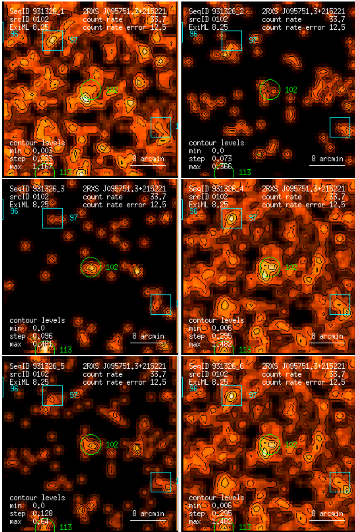
Figure 102: RASS 931326: detection 0102: band rate images, Gaussian filter: (1) PSPC channels 11 – 41, (2) 52 – 90, (3) 91 – 201, (4) 11 – 235, (5) 52 – 201, (6) 11 – 201. Broad band rates in counts/ks. Band rate contour levels in counts/ks/arcmin 2 .
