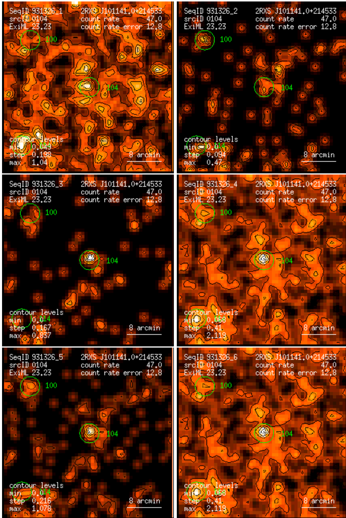
Figure 104: RASS 931326: detection 0104: band rate images, Gaussian filter: (1) PSPC channels 11 – 41, (2) 52 – 90, (3) 91 – 201, (4) 11 – 235, (5) 52 – 201, (6) 11 – 201. Broad band rates in counts/ks. Band rate contour levels in counts/ks/arcmin 2 .
