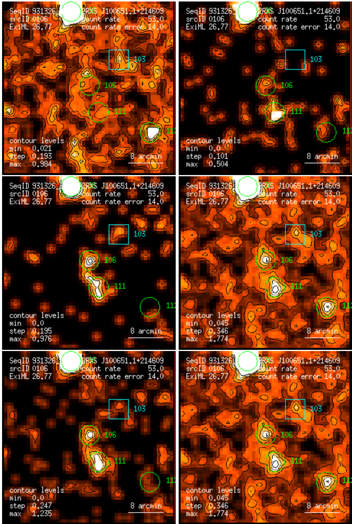
Figure 106: RASS 931326: detection 0106: band rate images, Gaussian filter: (1) PSPC channels 11 – 41, (2) 52 – 90, (3) 91 – 201, (4) 11 – 235, (5) 52 – 201, (6) 11 – 201. Broad band rates in counts/ks. Band rate contour levels in counts/ks/arcmin 2 .
