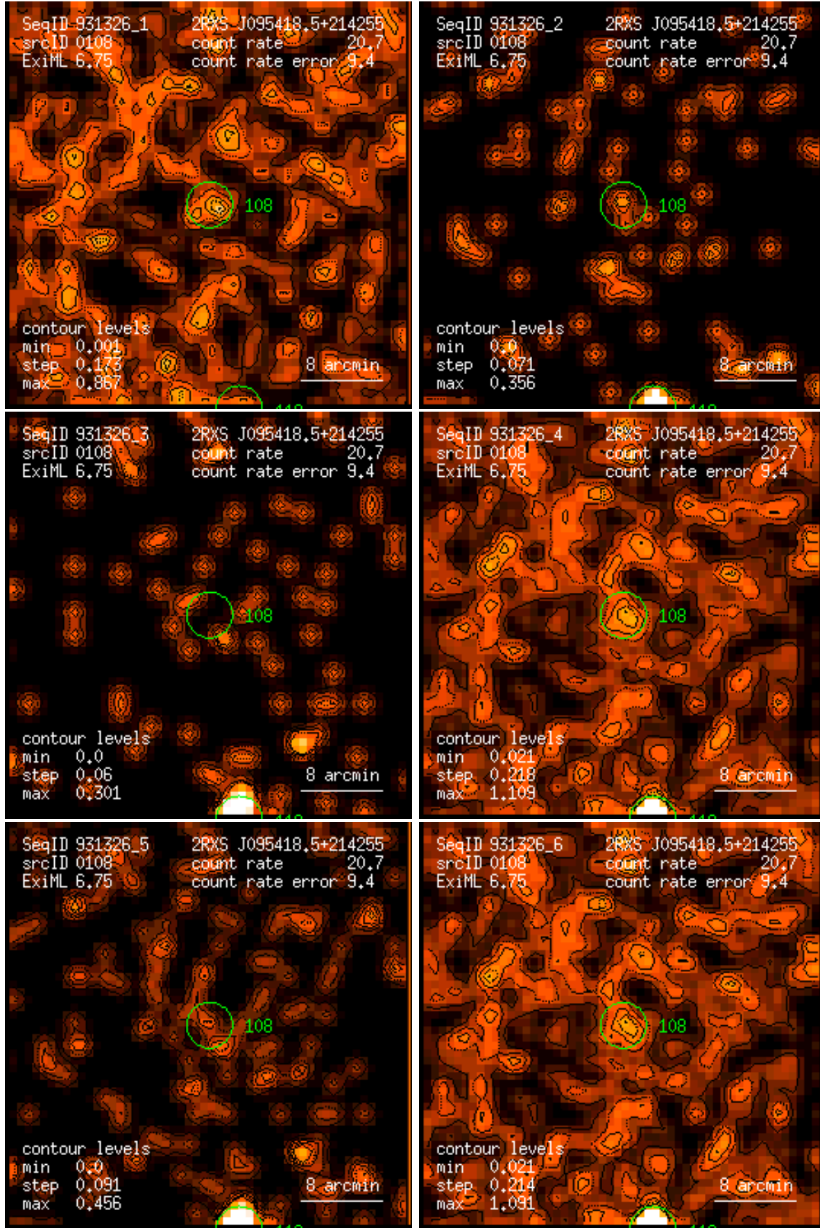
Figure 108: RASS 931326: detection 0108: band rate images, Gaussian filter: (1) PSPC channels 11 – 41, (2) 52 – 90, (3) 91 – 201, (4) 11 – 235, (5) 52 – 201, (6) 11 – 201. Broad band rates in counts/ks. Band rate contour levels in counts/ks/arcmin 2 .
