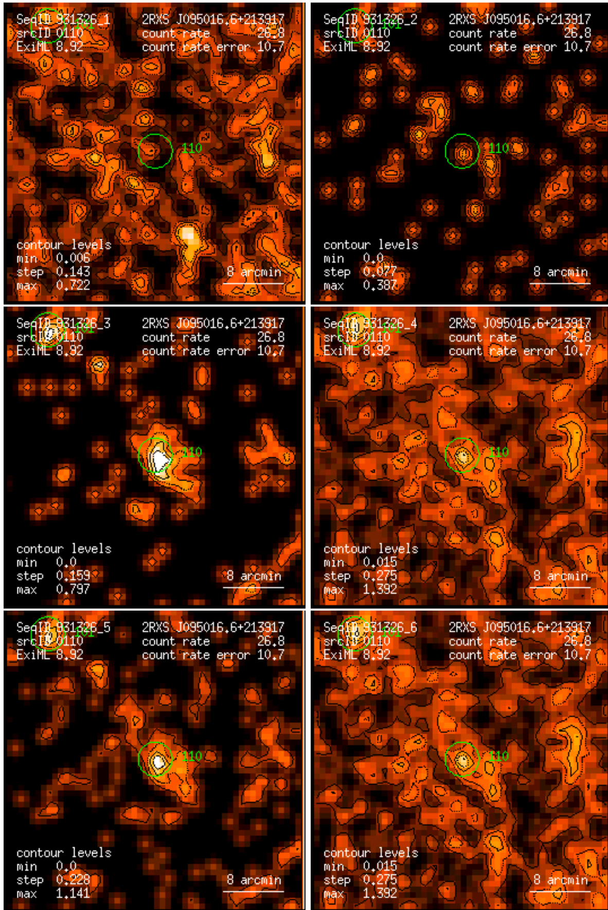
Figure 110: RASS 931326: detection 0110: band rate images, Gaussian filter: (1) PSPC channels 11 – 41, (2) 52 – 90, (3) 91 – 201, (4) 11 – 235, (5) 52 – 201, (6) 11 – 201. Broad band rates in counts/ks. Band rate contour levels in counts/ks/arcmin 2 .
