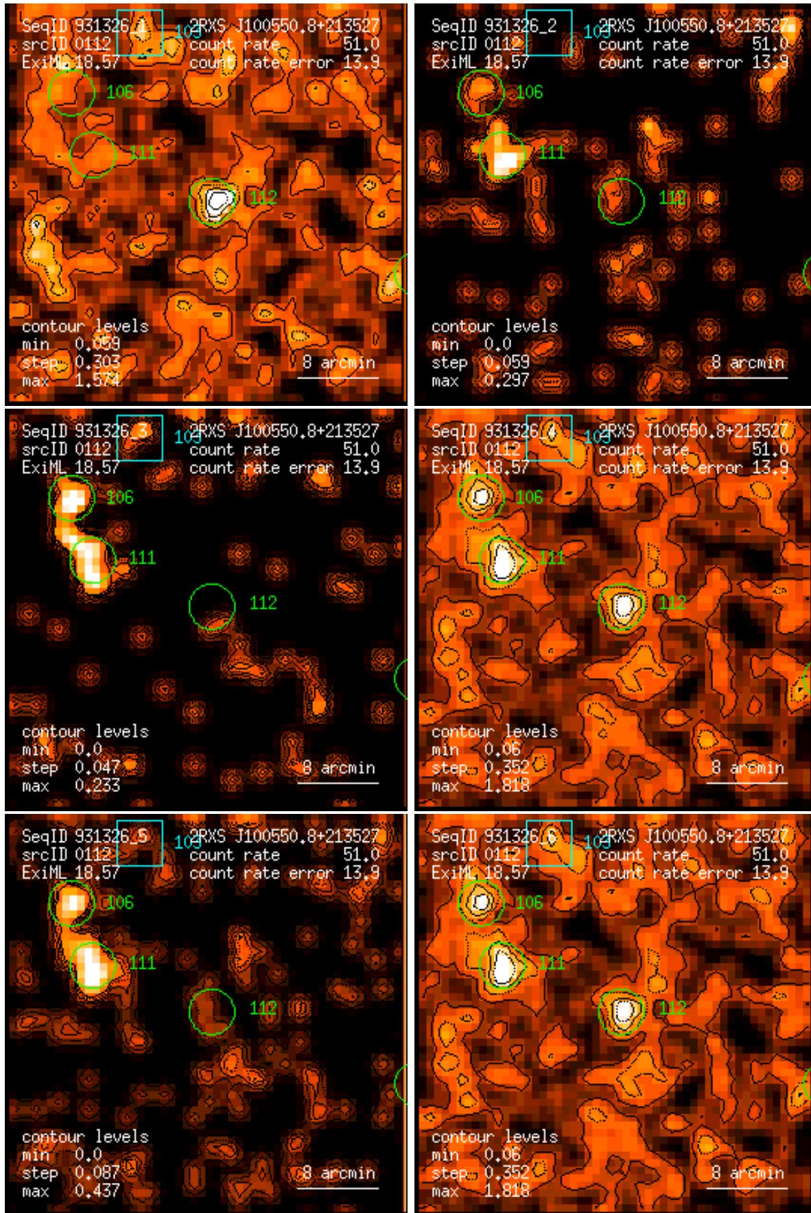
Figure 112: RASS 931326: detection 0112: band rate images, Gaussian filter: (1) PSPC channels 11 – 41, (2) 52 – 90, (3) 91 – 201, (4) 11 – 235, (5) 52 – 201, (6) 11 – 201. Broad band rates in counts/ks. Band rate contour levels in counts/ks/arcmin 2 .
