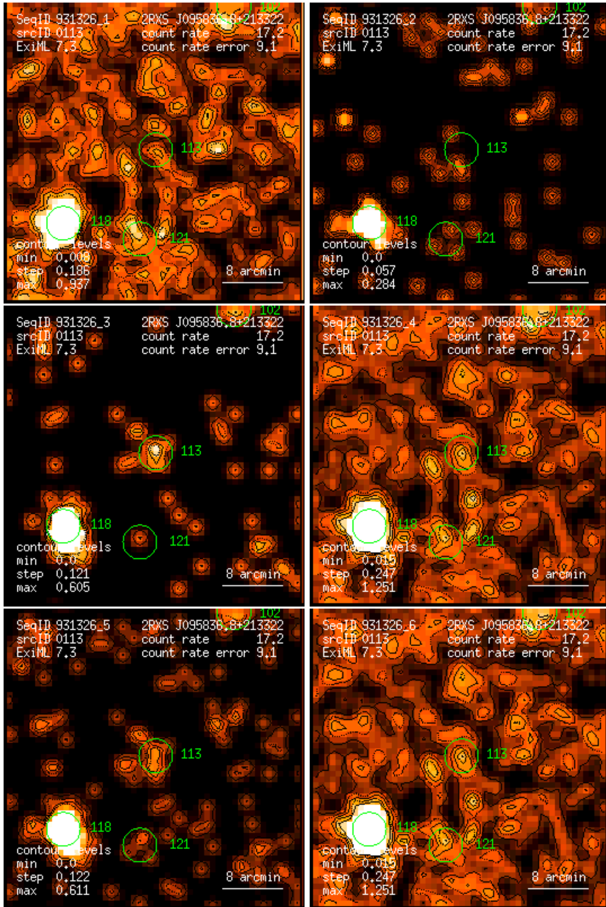
Figure 113: RASS 931326: detection 0113: band rate images, Gaussian filter: (1) PSPC channels 11 – 41, (2) 52 – 90, (3) 91 – 201, (4) 11 – 235, (5) 52 – 201, (6) 11 – 201. Broad band rates in counts/ks. Band rate contour levels in counts/ks/arcmin 2 .
