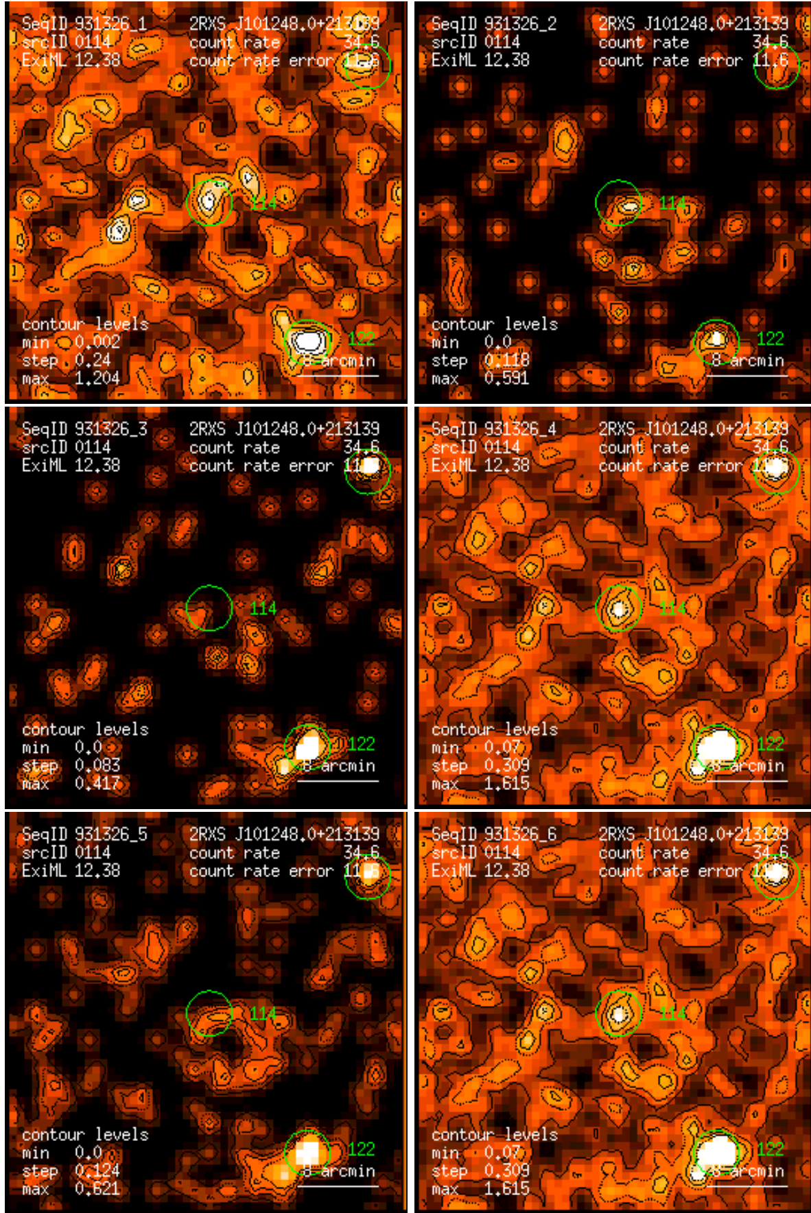
Figure 114: RASS 931326: detection 0114: band rate images, Gaussian filter: (1) PSPC channels 11 – 41, (2) 52 – 90, (3) 91 – 201, (4) 11 – 235, (5) 52 – 201, (6) 11 – 201. Broad band rates in counts/ks. Band rate contour levels in counts/ks/arcmin 2 .
