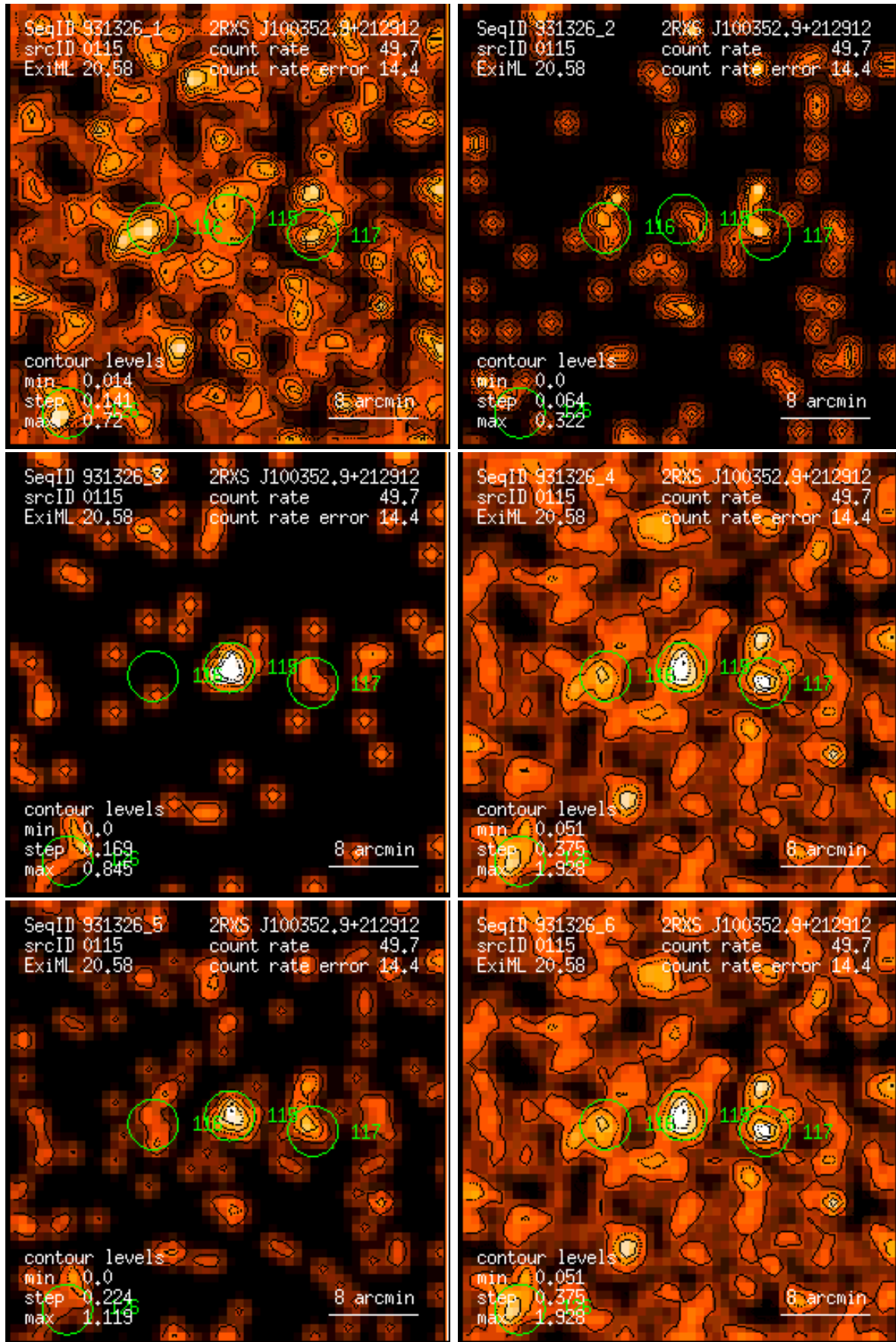
Figure 115: RASS 931326: detection 0115: band rate images, Gaussian filter: (1) PSPC channels 11 – 41, (2) 52 – 90, (3) 91 – 201, (4) 11 – 235, (5) 52 – 201, (6) 11 – 201. Broad band rates in counts/ks. Band rate contour levels in counts/ks/arcmin 2 .
