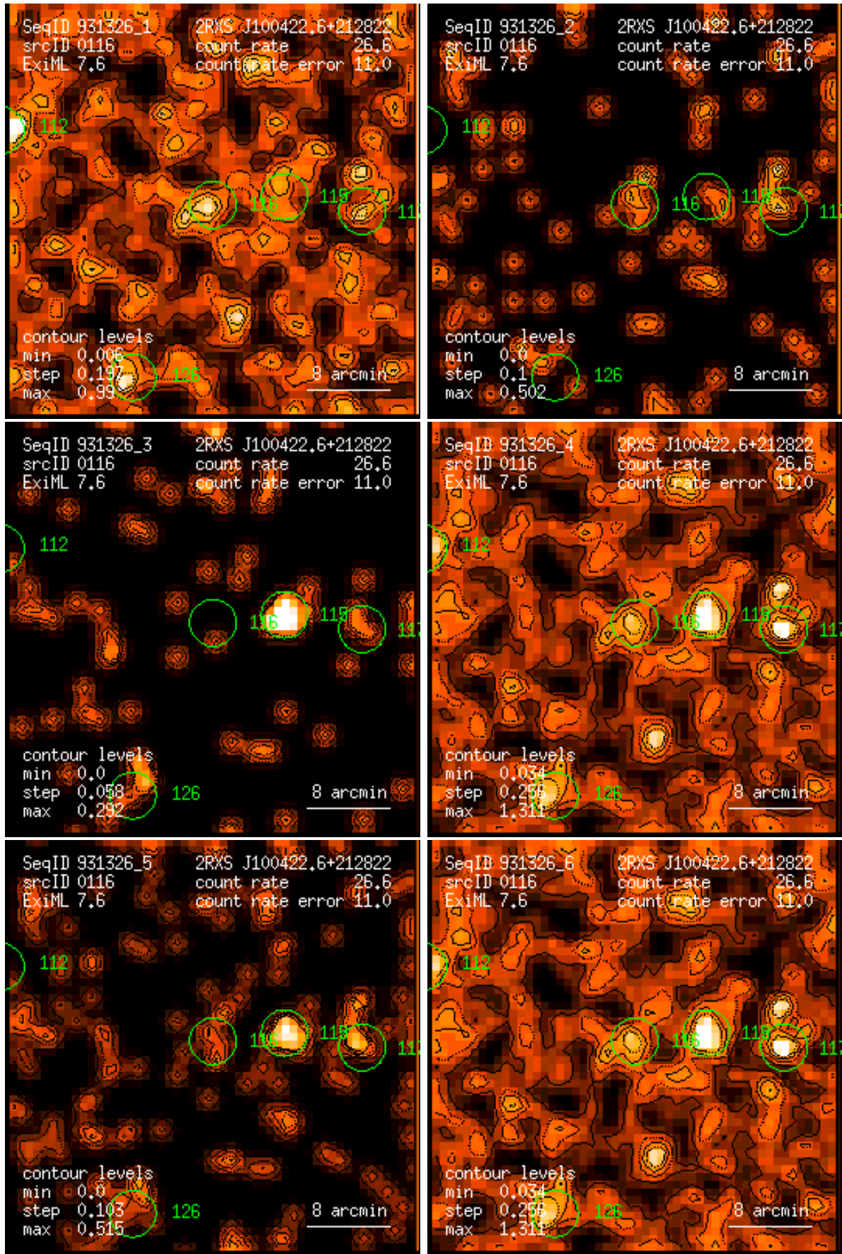
Figure 116: RASS 931326: detection 0116: band rate images, Gaussian filter: (1) PSPC channels 11 – 41, (2) 52 – 90, (3) 91 – 201, (4) 11 – 235, (5) 52 – 201, (6) 11 – 201. Broad band rates in counts/ks. Band rate contour levels in counts/ks/arcmin 2 .
