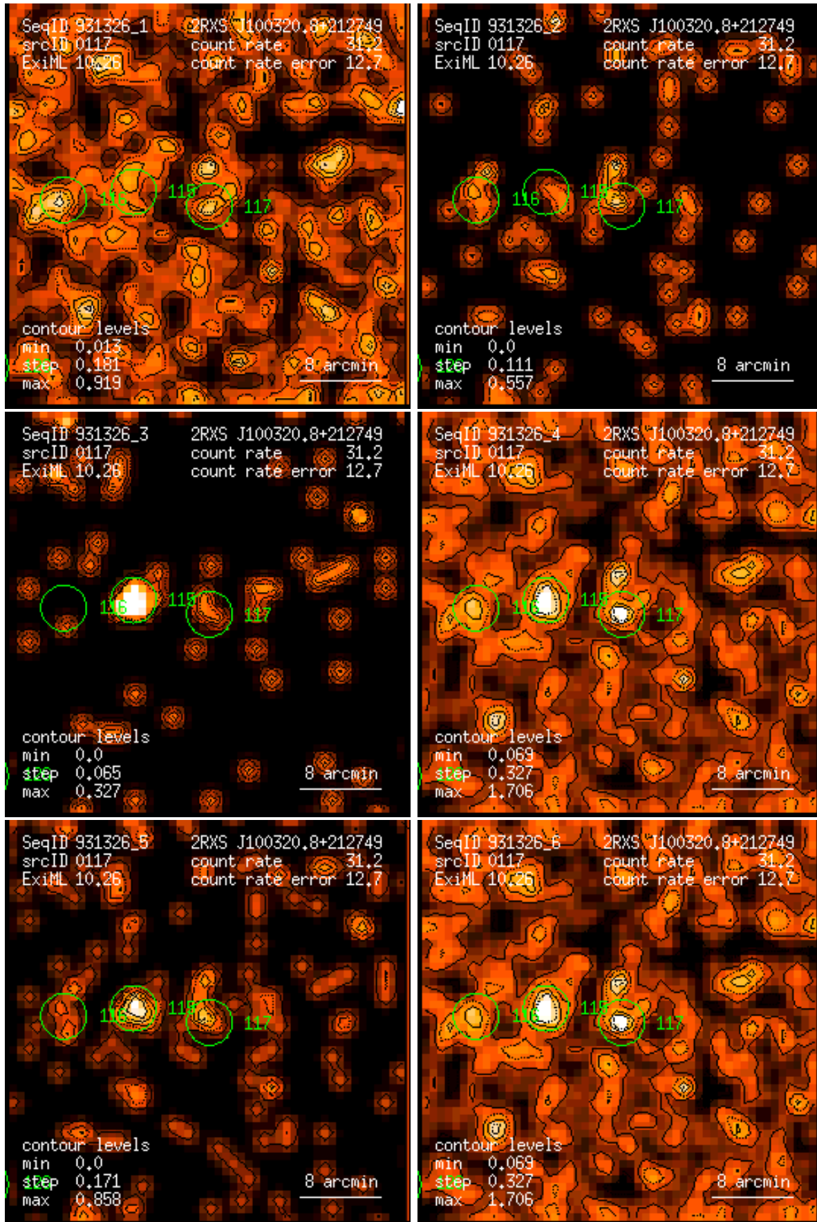
Figure 117: RASS 931326: detection 0117: band rate images, Gaussian filter: (1) PSPC channels 11 – 41, (2) 52 – 90, (3) 91 – 201, (4) 11 – 235, (5) 52 – 201, (6) 11 – 201. Broad band rates in counts/ks. Band rate contour levels in counts/ks/arcmin 2 .
