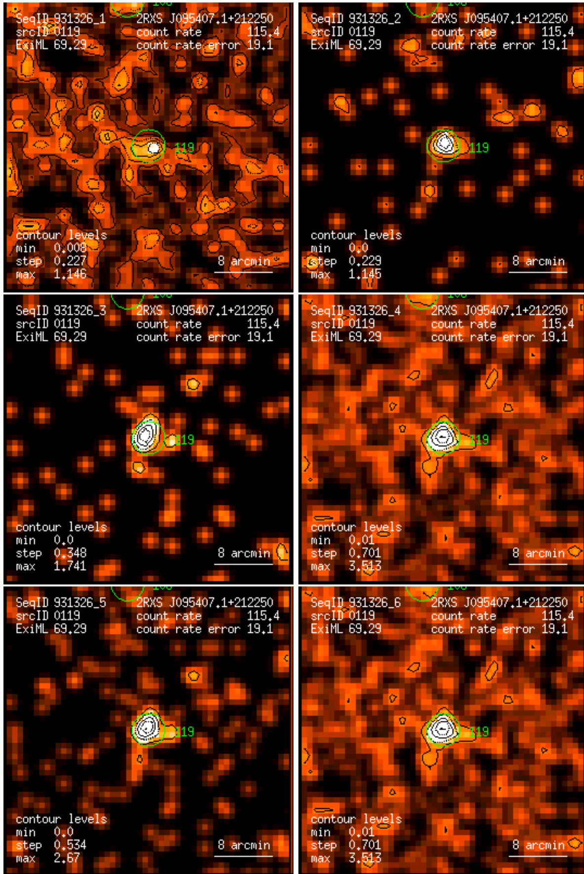
Figure 119: RASS 931326: detection 0119: band rate images, Gaussian filter: (1) PSPC channels 11 – 41, (2) 52 – 90, (3) 91 – 201, (4) 11 – 235, (5) 52 – 201, (6) 11 – 201. Broad band rates in counts/ks. Band rate contour levels in counts/ks/arcmin 2 .
