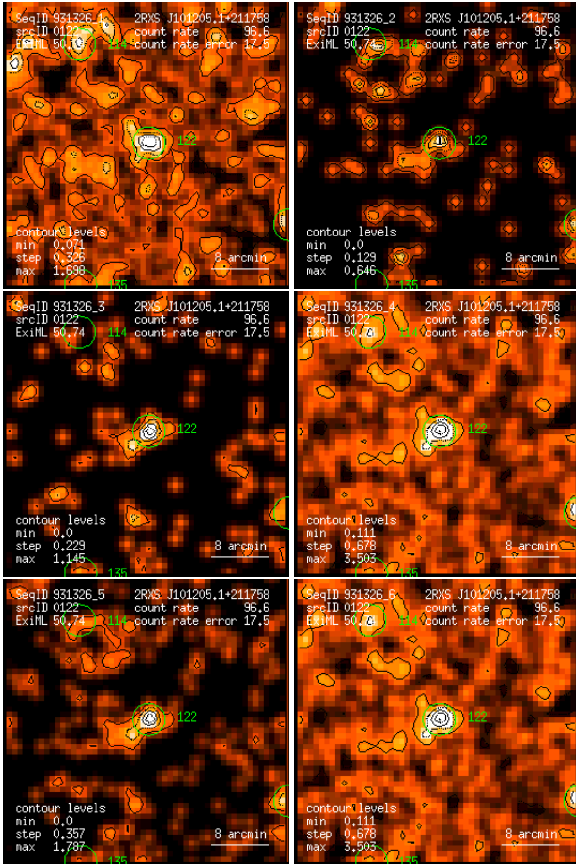
Figure 122: RASS 931326: detection 0122: band rate images, Gaussian filter: (1) PSPC channels 11 – 41, (2) 52 – 90, (3) 91 – 201, (4) 11 – 235, (5) 52 – 201, (6) 11 – 201. Broad band rates in counts/ks. Band rate contour levels in counts/ks/arcmin 2 .
