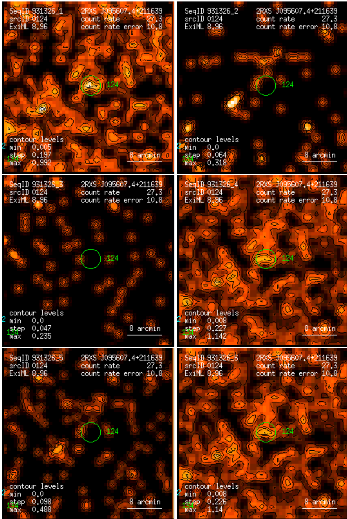
Figure 124: RASS 931326: detection 0124: band rate images, Gaussian filter: (1) PSPC channels 11 – 41, (2) 52 – 90, (3) 91 – 201, (4) 11 – 235, (5) 52 – 201, (6) 11 – 201. Broad band rates in counts/ks. Band rate contour levels in counts/ks/arcmin 2 .
