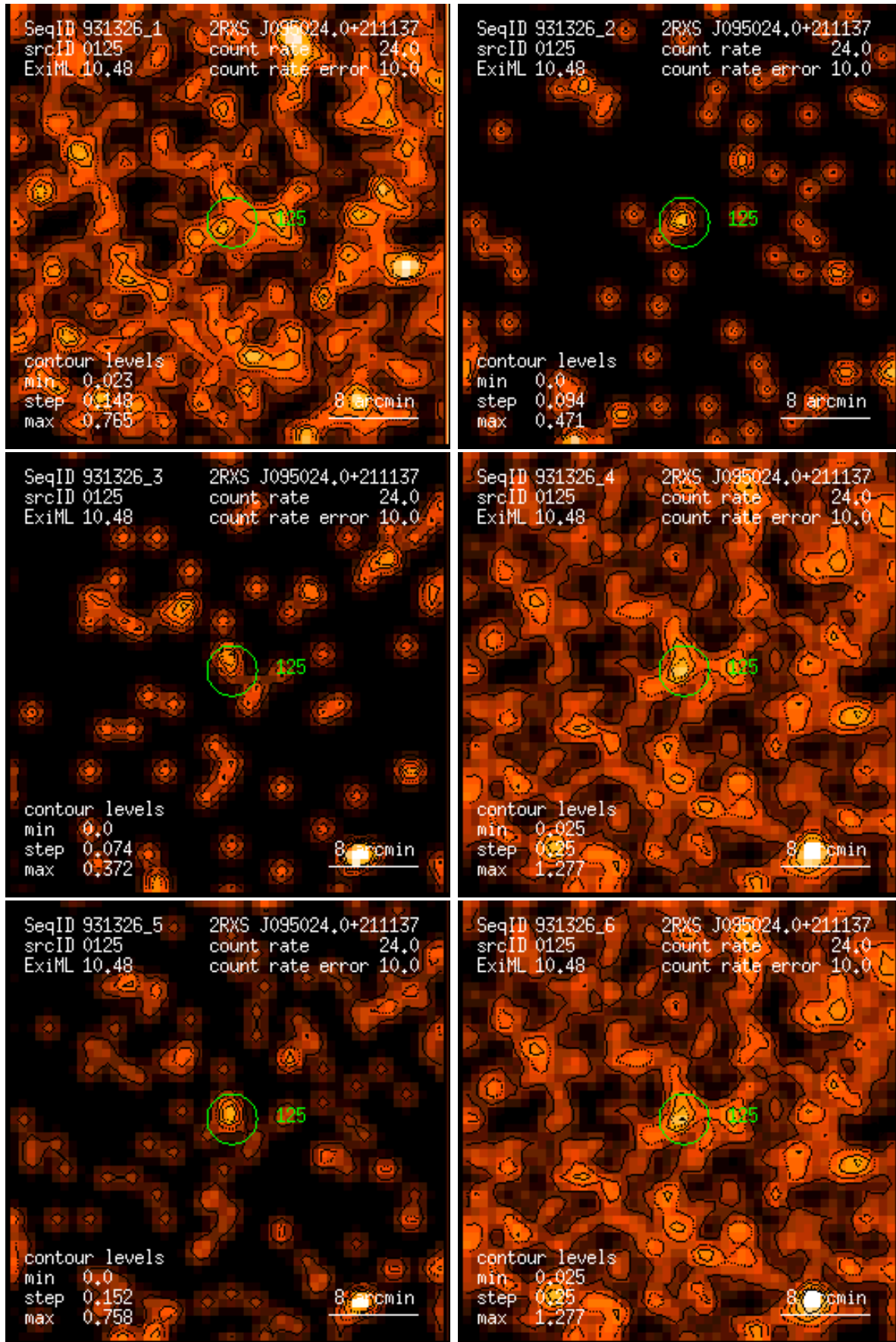
Figure 125: RASS 931326: detection 0125: band rate images, Gaussian filter: (1) PSPC channels 11 – 41, (2) 52 – 90, (3) 91 – 201, (4) 11 – 235, (5) 52 – 201, (6) 11 – 201. Broad band rates in counts/ks. Band rate contour levels in counts/ks/arcmin 2 .
