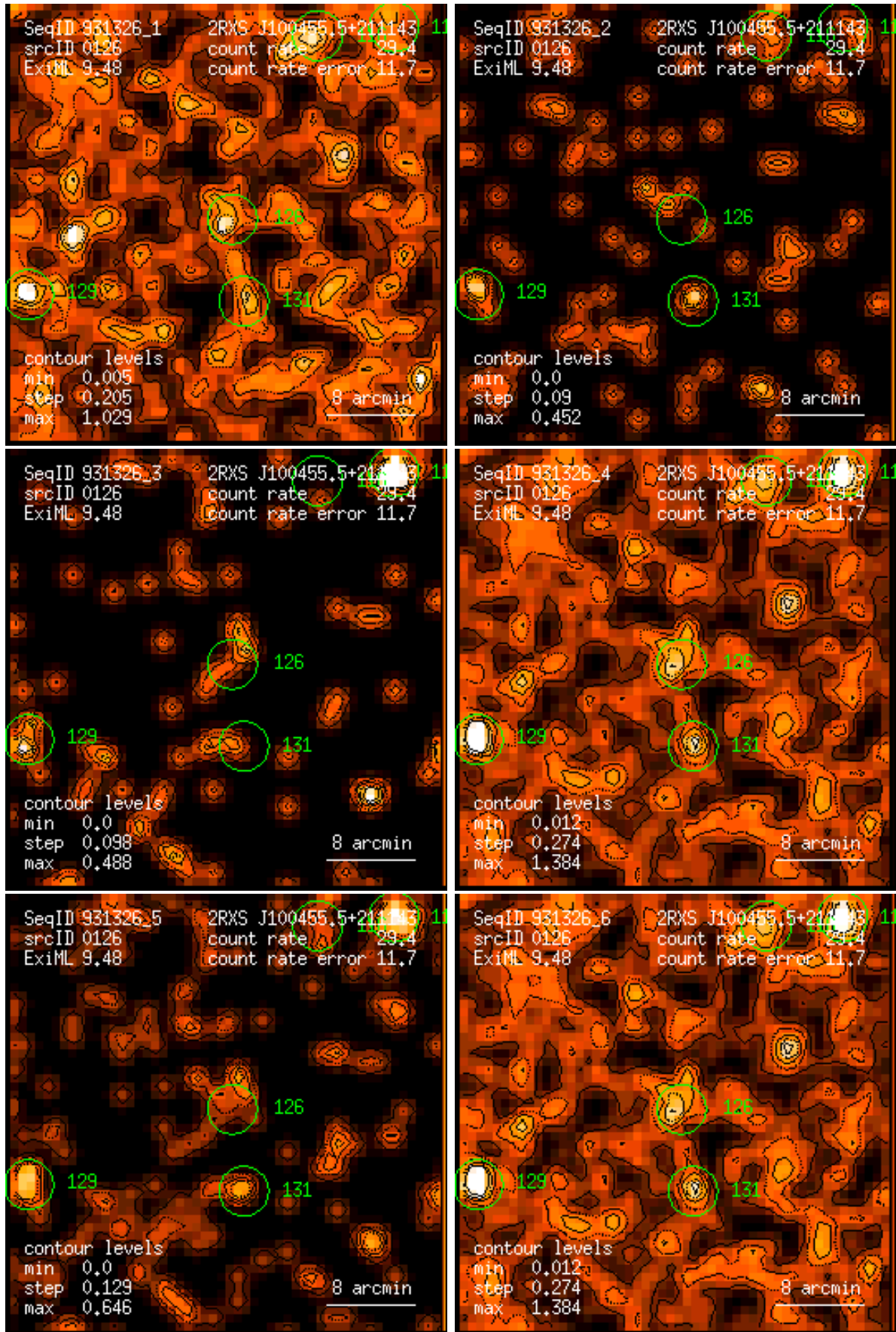
Figure 126: RASS 931326: detection 0126: band rate images, Gaussian filter: (1) PSPC channels 11 – 41, (2) 52 – 90, (3) 91 – 201, (4) 11 – 235, (5) 52 – 201, (6) 11 – 201. Broad band rates in counts/ks. Band rate contour levels in counts/ks/arcmin 2 .
