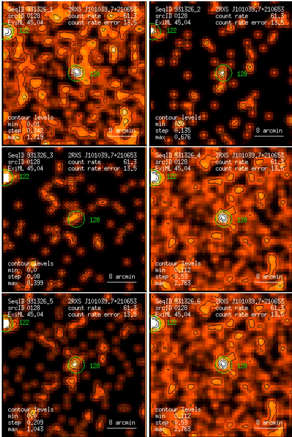
Figure 128: RASS 931326: detection 0128: band rate images, Gaussian filter: (1) PSPC channels 11 – 41, (2) 52 – 90, (3) 91 – 201, (4) 11 – 235, (5) 52 – 201, (6) 11 – 201. Broad band rates in counts/ks. Band rate contour levels in counts/ks/arcmin 2 .
