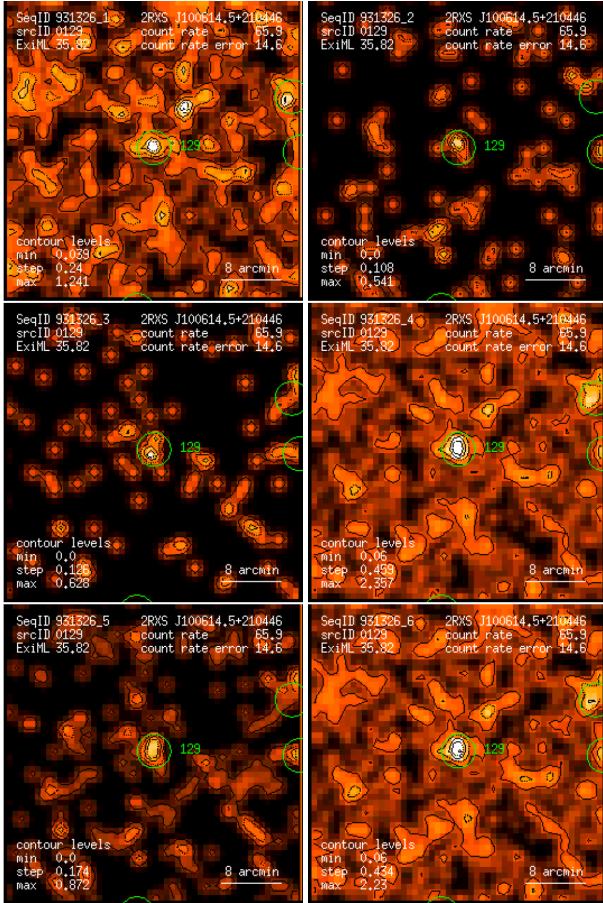
Figure 129: RASS 931326: detection 0129: band rate images, Gaussian filter: (1) PSPC channels 11 – 41, (2) 52 – 90, (3) 91 – 201, (4) 11 – 235, (5) 52 – 201, (6) 11 – 201. Broad band rates in counts/ks. Band rate contour levels in counts/ks/arcmin 2 .
